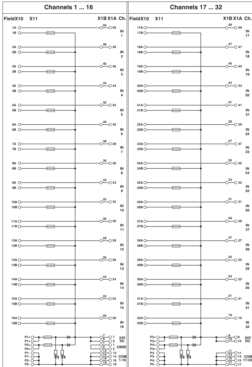
Circuit diagram
