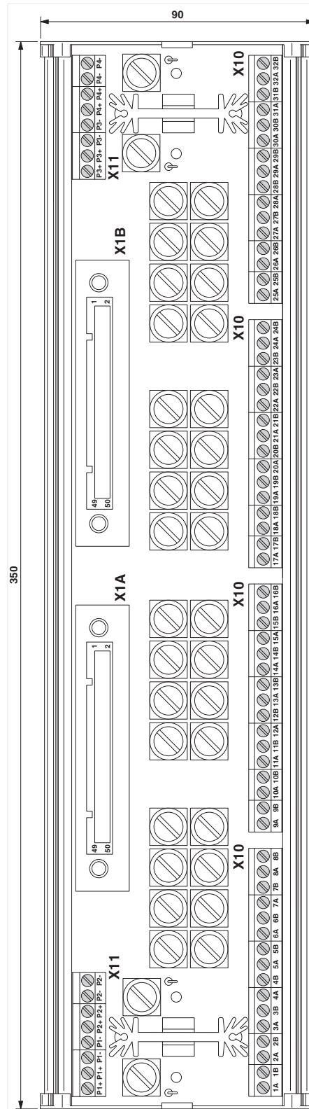
Dimensioned drawing
