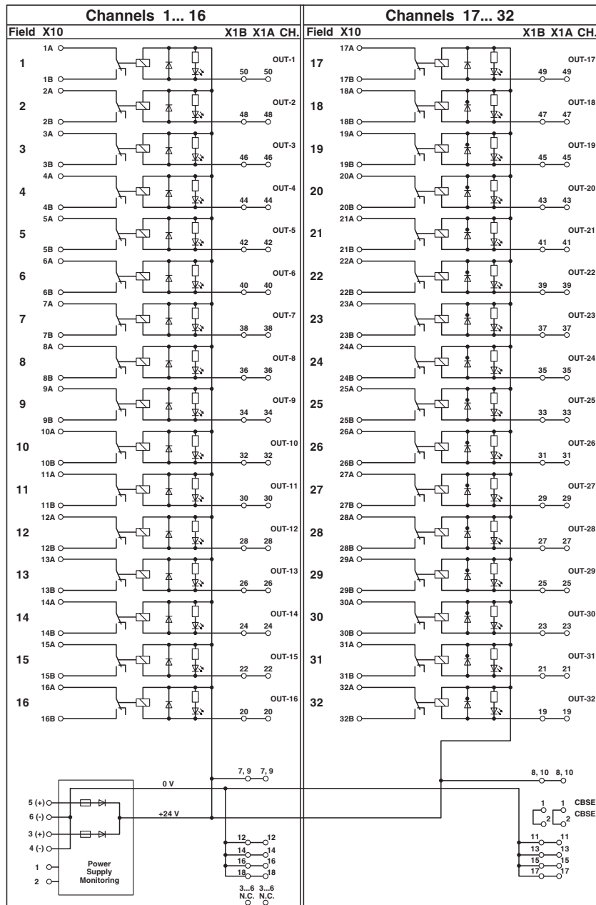
Circuit diagram
