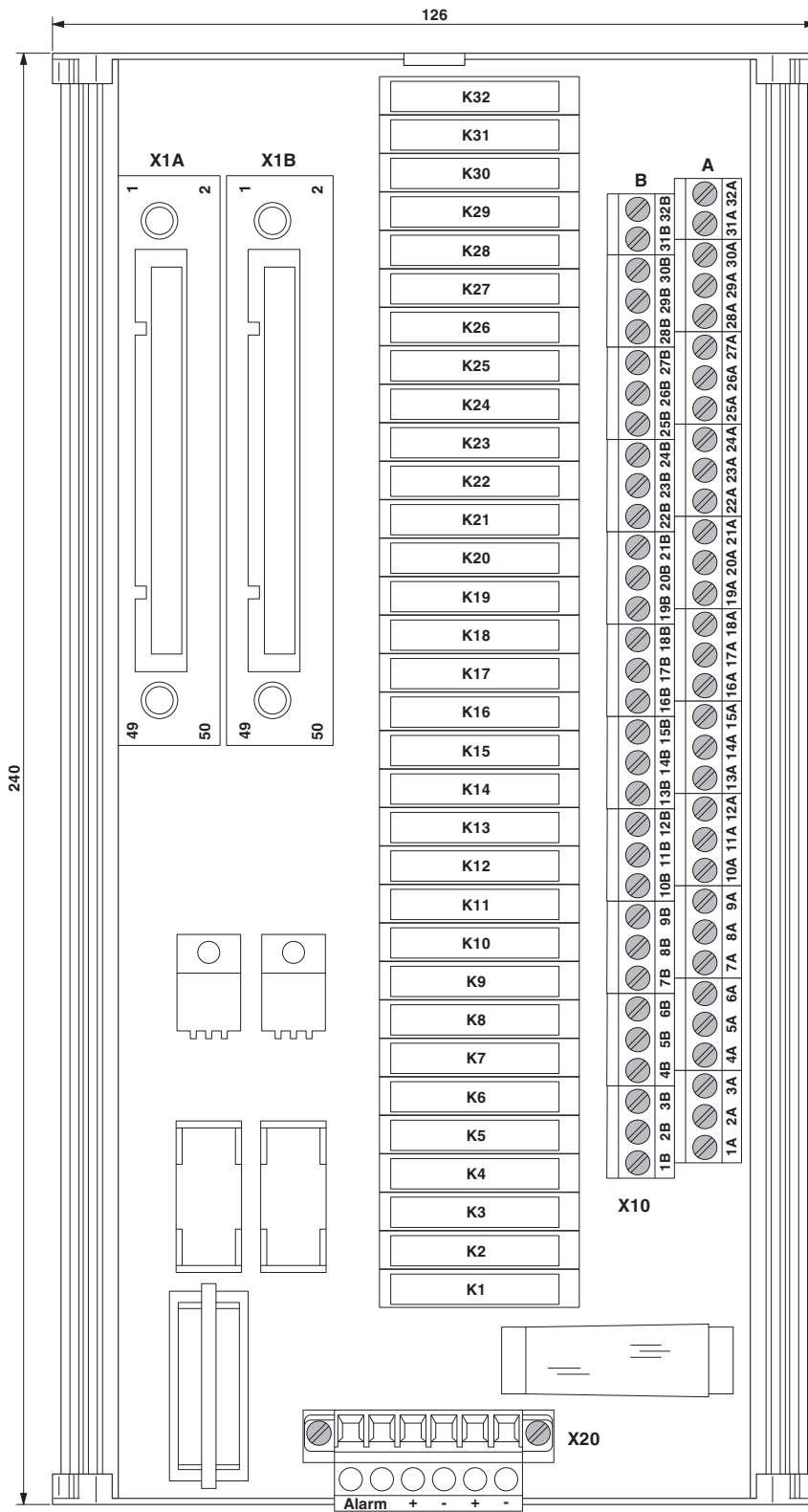
Dimensioned drawing
