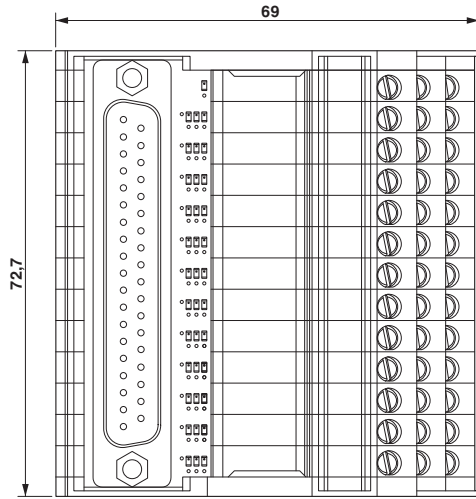
Dimensioned drawing
