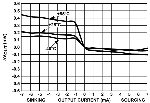
FIGURE 23. LOAD REGULATION OVER-TEMPERATURE
