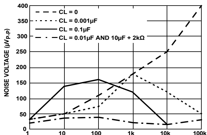
FIGURE 118. NOISE REDUCTION
