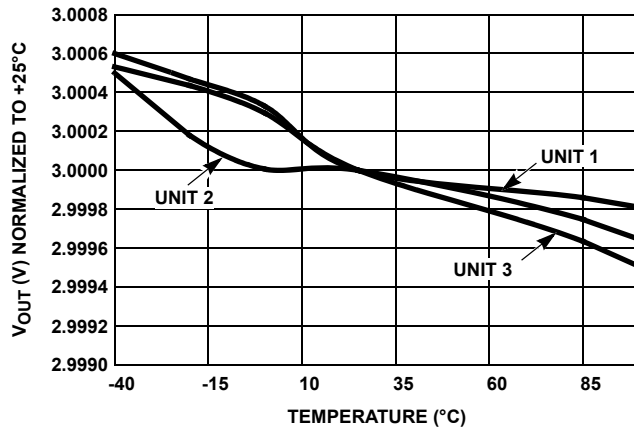
FIGURE 86. V_{OUT} vs TEMPERATURE NORMALIZED TO +25°C
