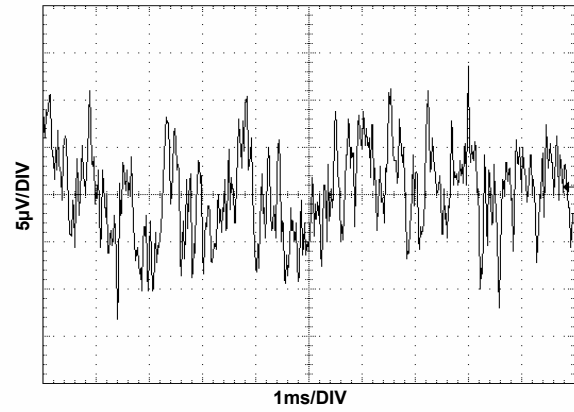
FIGURE 56. V_{OUT} NOISE
