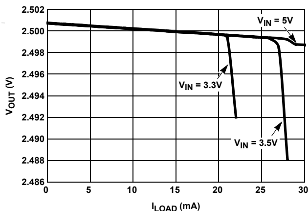
FIGURE 115. DIFFERENT V_{IN} AT ROOM TEMPERATURE
