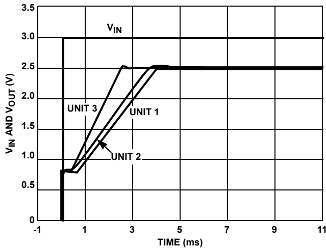
FIGURE 120. TURN-ON TIME
