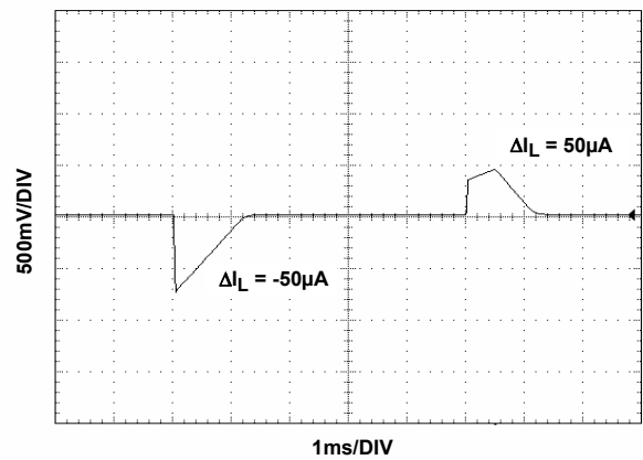
FIGURE 52. LOAD TRANSIENT RESPONSE
