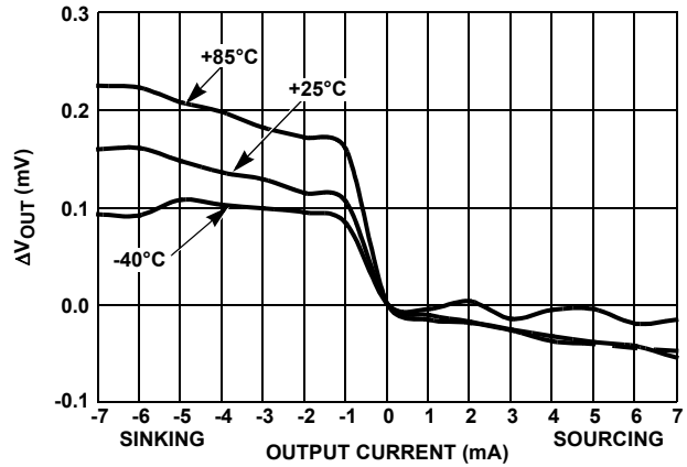
FIGURE 37. LOAD REGULATION
