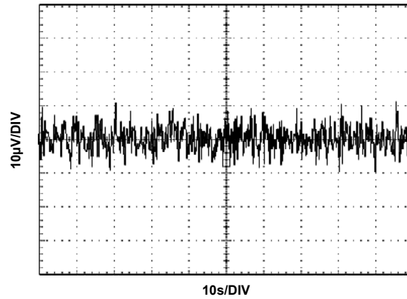
FIGURE 42. V_{OUT} NOISE
