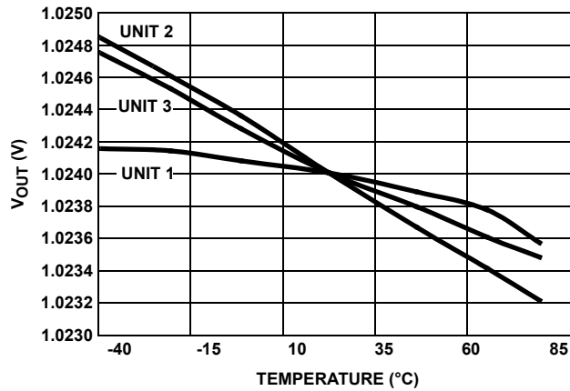
FIGURE 6. V_{OUT} vs TEMPERATURE NORMALIZED to +25^\circ C
