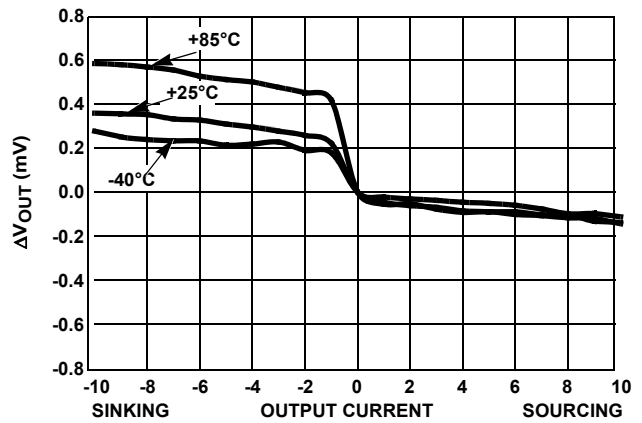
FIGURE 50. LOAD REGULATION OVER-TEMPERATURE
