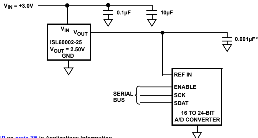
FIGURE 1. TYPICAL APPLICATION
