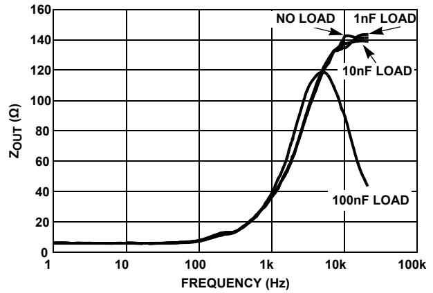
FIGURE 98. Z_{OUT} vs FREQUENCY
