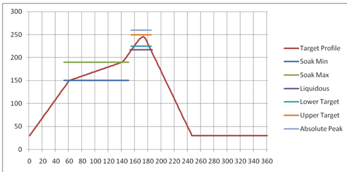
Figure 12: Recommended Reflow Temperature
