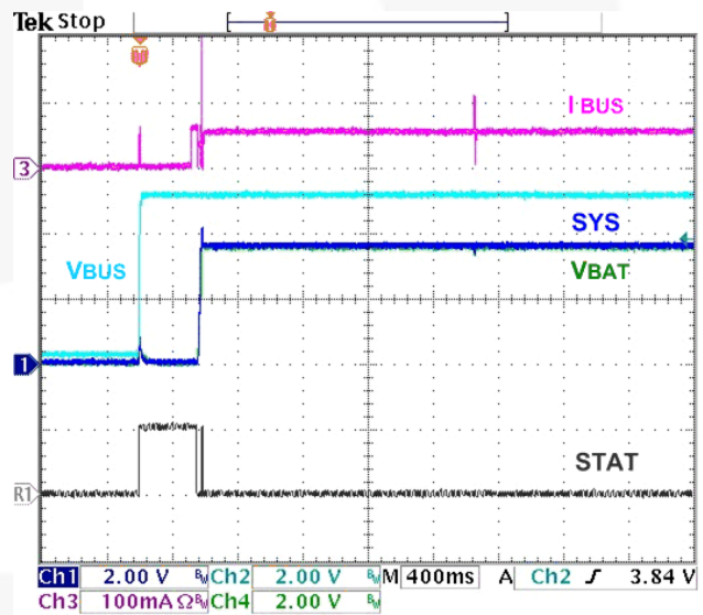
Figure 18. No Battery at V BUS Power-Up, FAN54042, 100 Ω SYS Load, 1 kΩ V BAT Load
