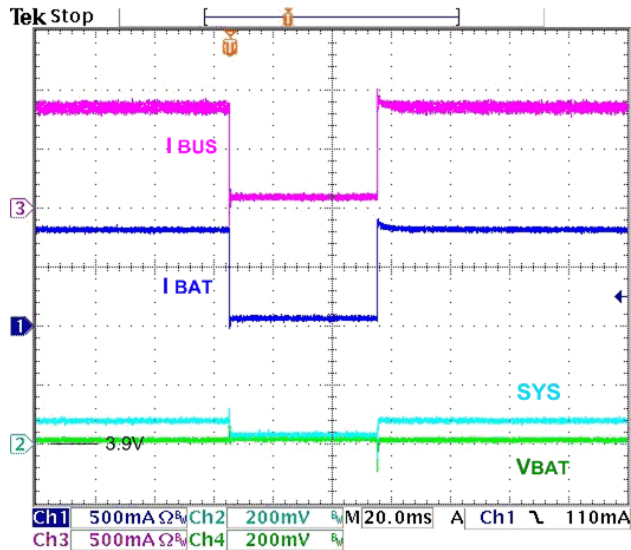
Figure 15. Battery Removal / Insertion while Charging, TE=0, 3.9 V BAT , I CHRG =950 mA, I BUSLIM =No Limit, 50 Ω SYS Load
