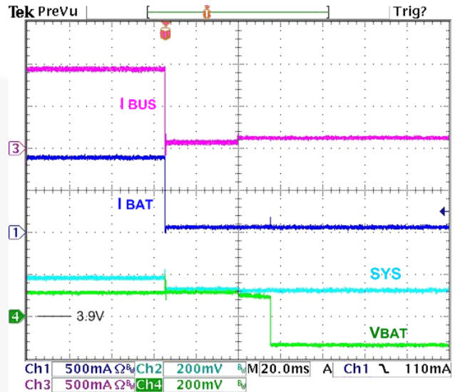
Figure 16. Battery Removal / Insertion when Charging, TE=1, 3.9 V BAT , I CHRG =950 mA, I BUSLIM =No Limit, 50 Ω SYS Load
