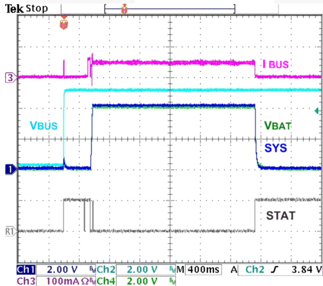
Figure 17. No Battery at V BUS Power-Up, FAN54040, 100 Ω SYS Load, 1 kΩ V BAT Load
