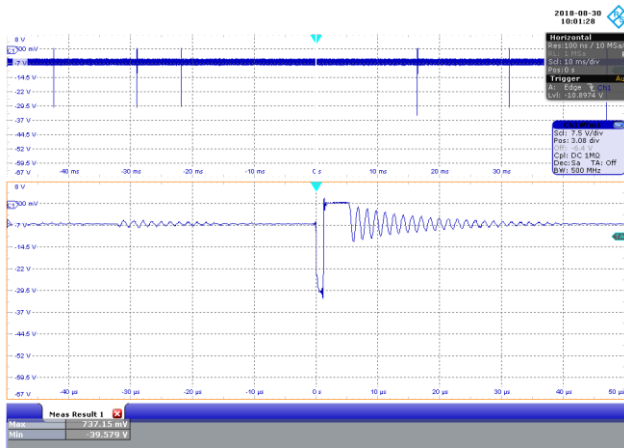
Figure 89 – 230 VAC 50 Hz, No-Load. CH1: 12 V F WL DIODE , 7.5 V / div., 10 ms / div. Zoom: 10 µs / div. 12 V PIV MAX = 39.579 V.
