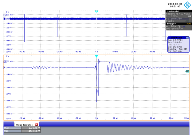
Figure 90 – 277 VAC 50 Hz, No-Load. CH1: 12 V F WL DIODE , 7.5 V / div., 10 ms / div. Zoom: 10 µs / div. 12 V PIV MAX = 45.211 V.
