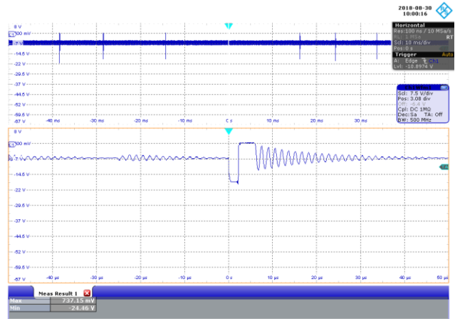
Figure 88 – 115 VAC 60 Hz, No-Load. CH1: 12 V F WL DIODE , 7.5 V / div., 10 ms / div. Zoom: 10 µs / div. 12 V PIV MAX = 24.46 V.
