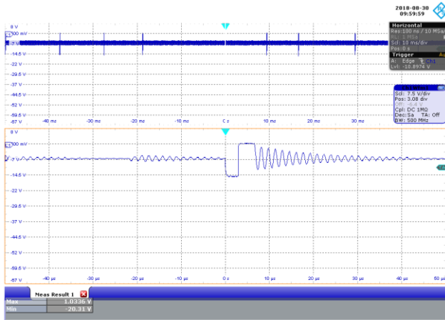
Figure 87 – 85 VAC 60 Hz, No-Load. CH1: 12 V F WL DIODE , 7.5 V / div., 10 ms / div. Zoom: 10 µs / div. 12 V PIV MAX = 20.31 V.
