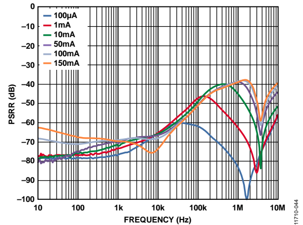
Figure 44. LDO PSRR Across Output Load, V_{VIN3} = 5.0V , V_{VOUT3} = 3.0V
