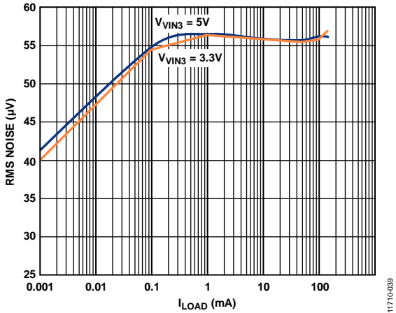
Figure 39. LDO Output Noise vs. Load Current, Across Input Voltage, V_{VIN3} = 3.3V , V_{VOUT3} = 2.8V
