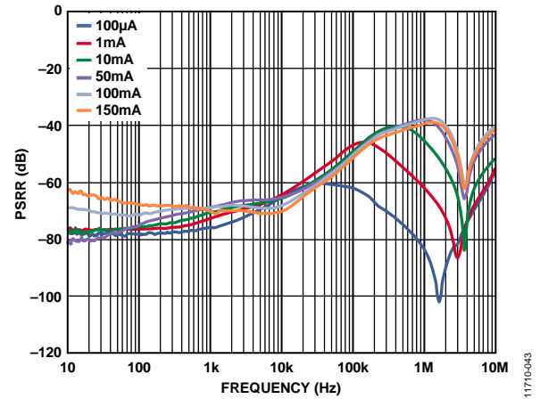
Figure 43. LDO PSRR Across Output Load, V_{VIN3} = 5.0V , V_{VOUT3} = 2.8V
