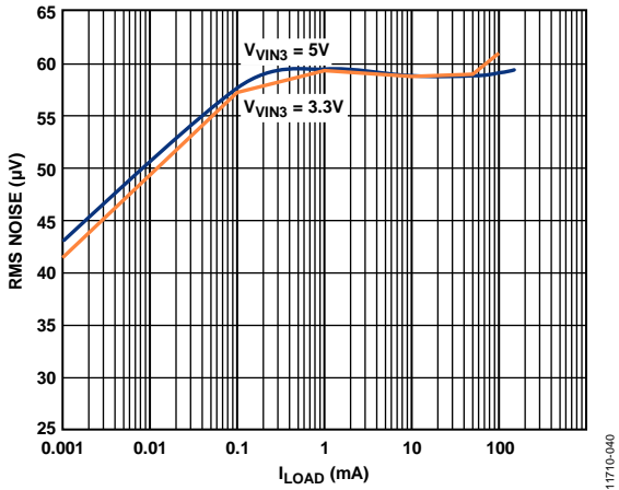
Figure 40. LDO Output Noise vs. Load Current, Across Input Voltage, V_{VIN3} = 3.3V , V_{VOUT3} = 3.0V
