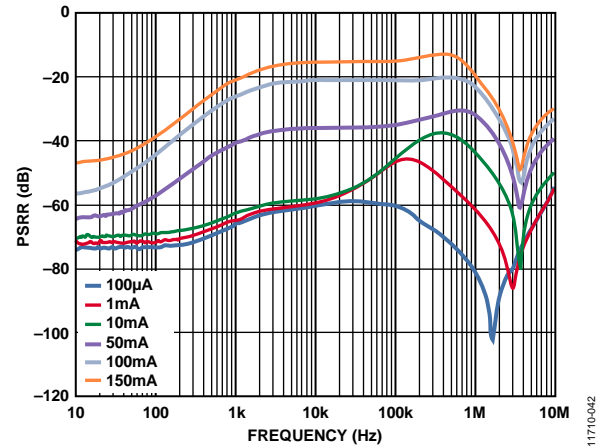
Figure 42. LDO PSRR Across Output Load, V_{VIN3} = 3.3V , V_{VOUT3} = 3.0V
