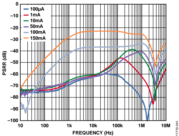
Figure 41. LDO PSRR Across Output Load, V_{VIN3} = 3.3V , V_{VOUT3} = 2.8V
