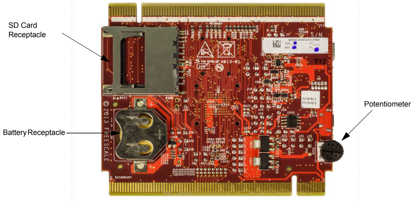
Figure 2. Back side of TWR-K64F120M
