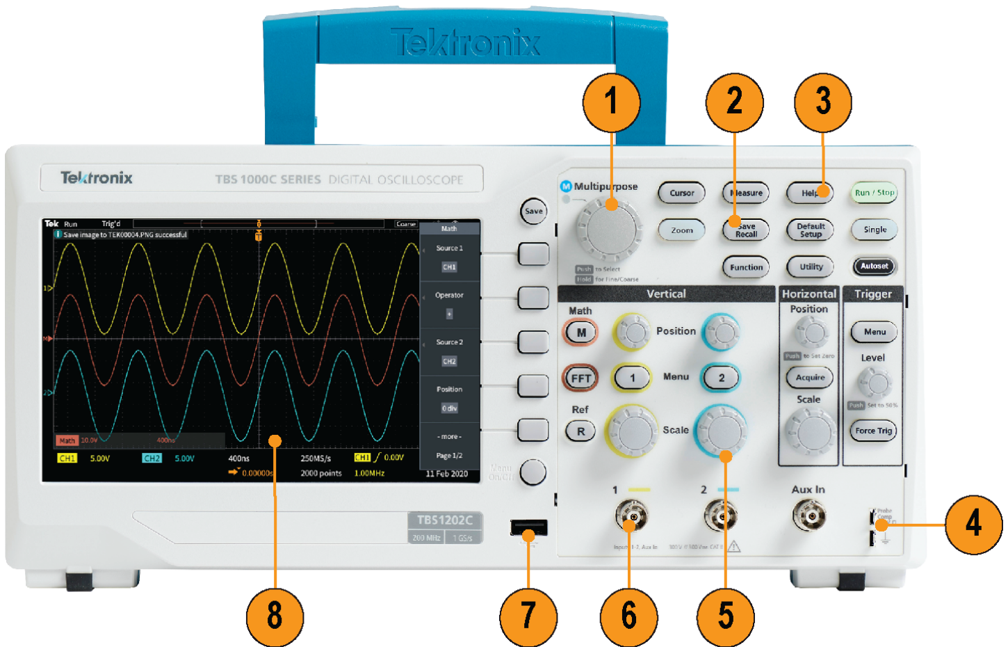
TBS1000C front panel
