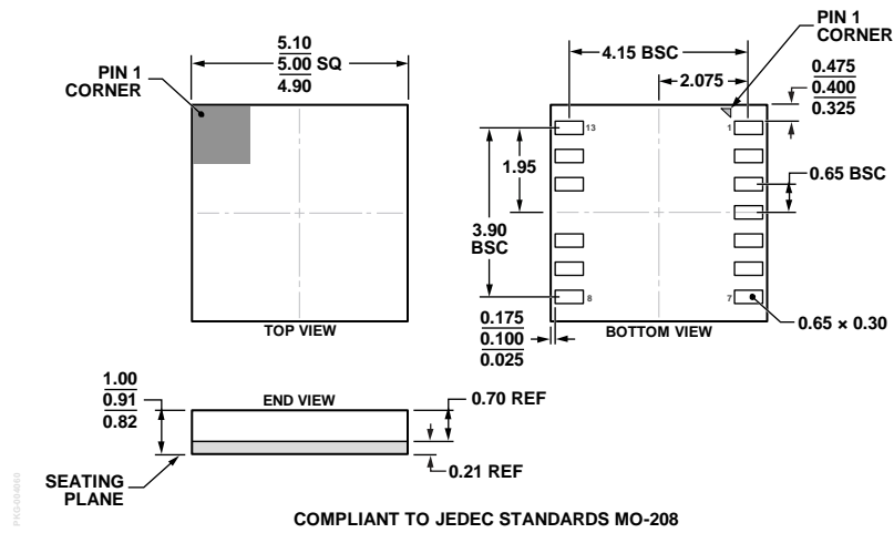
COMPLIANT TO JEDEC STANDARDS MO-208 Figure 23. 13-Terminal Land Grid Array [LGA] (CC-13-1) Dimensions shown in millimeters
