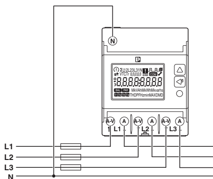
Connection diagram
