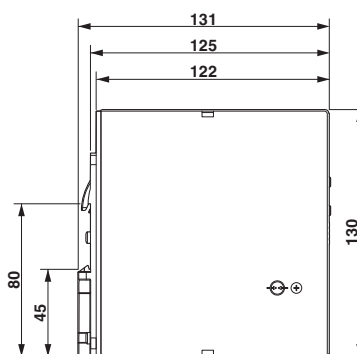
Dimensional drawing
