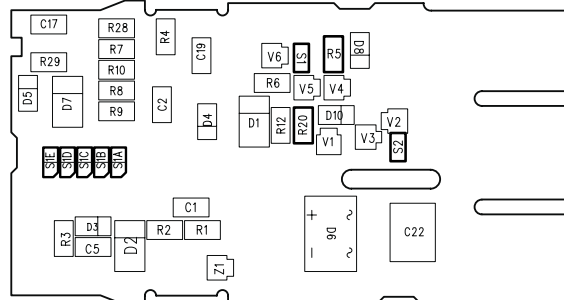
power HV RR sealing side (HV RD)
