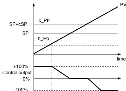
Control output with proportional action only if proportional heating band overlaps proportional cooling band.
