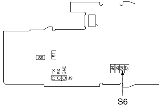
CPU BOARD (Sealing Side) S6 = ON Enable Calibration
