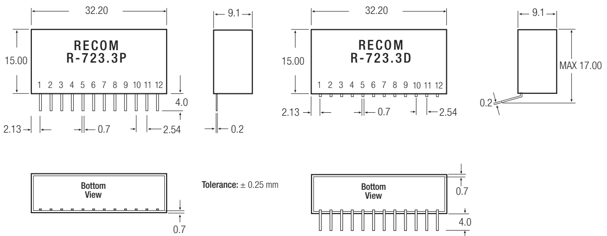
Pin Connections
