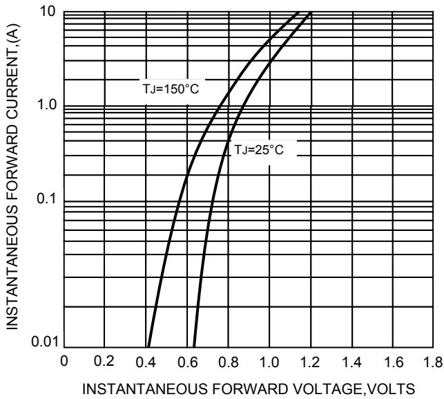
FIG.3-TYPICAL FORWARD CHARACTERISTICS
