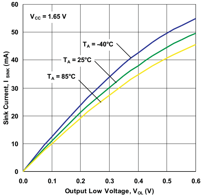
OUTPUT LOW VOLTAGE vs I/O SINK CURRENT
