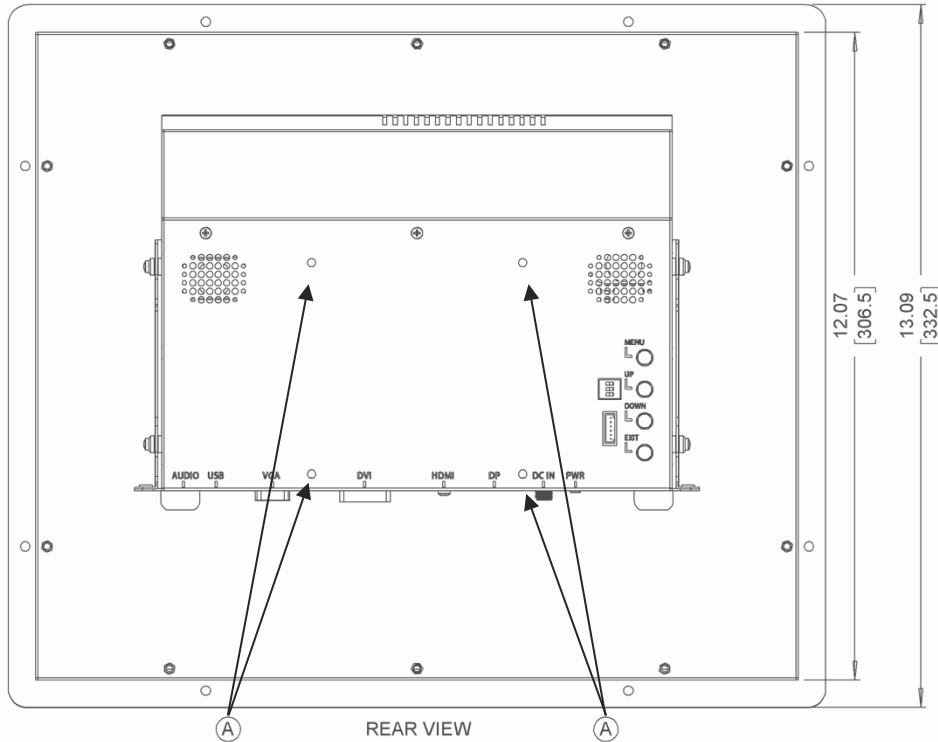
REAR VIEW
