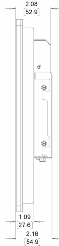
SIDE VIEW
