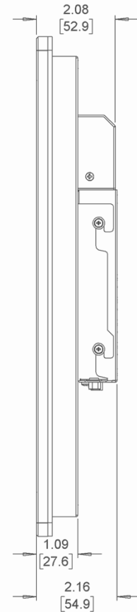
SIDE VIEW
