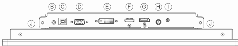
BOTTOM VIEW
