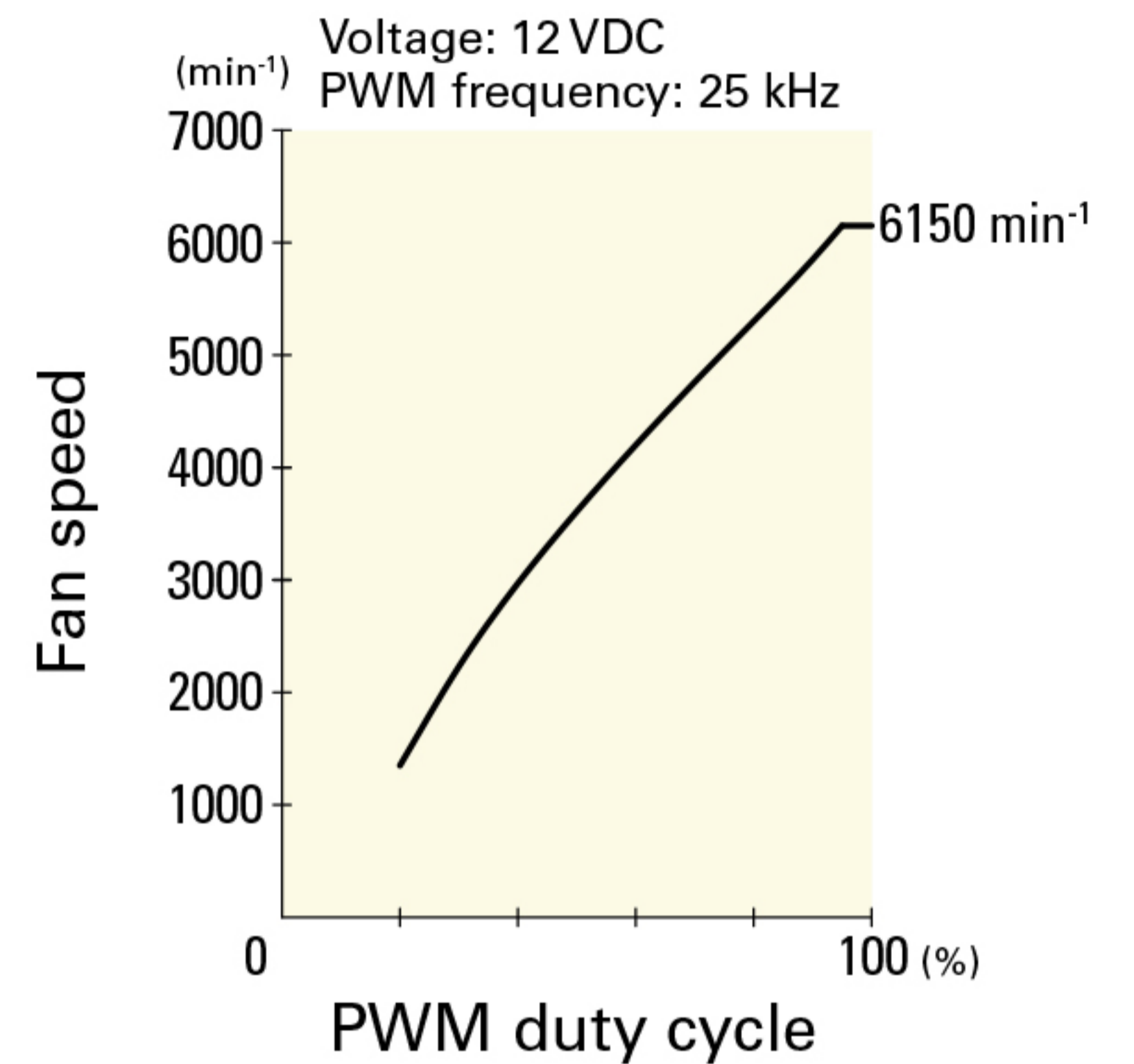
PWM duty - Speed characteristics example
