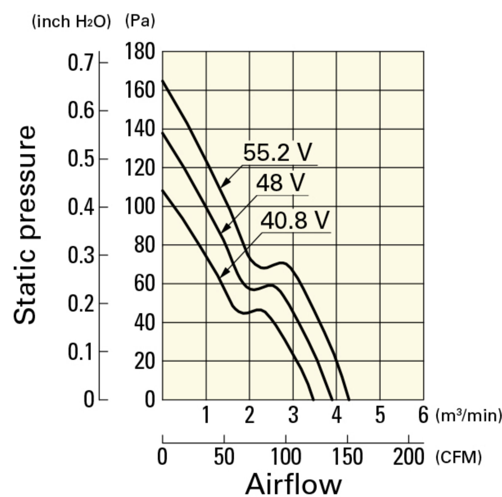
9G1248F101 With pulse sensor
