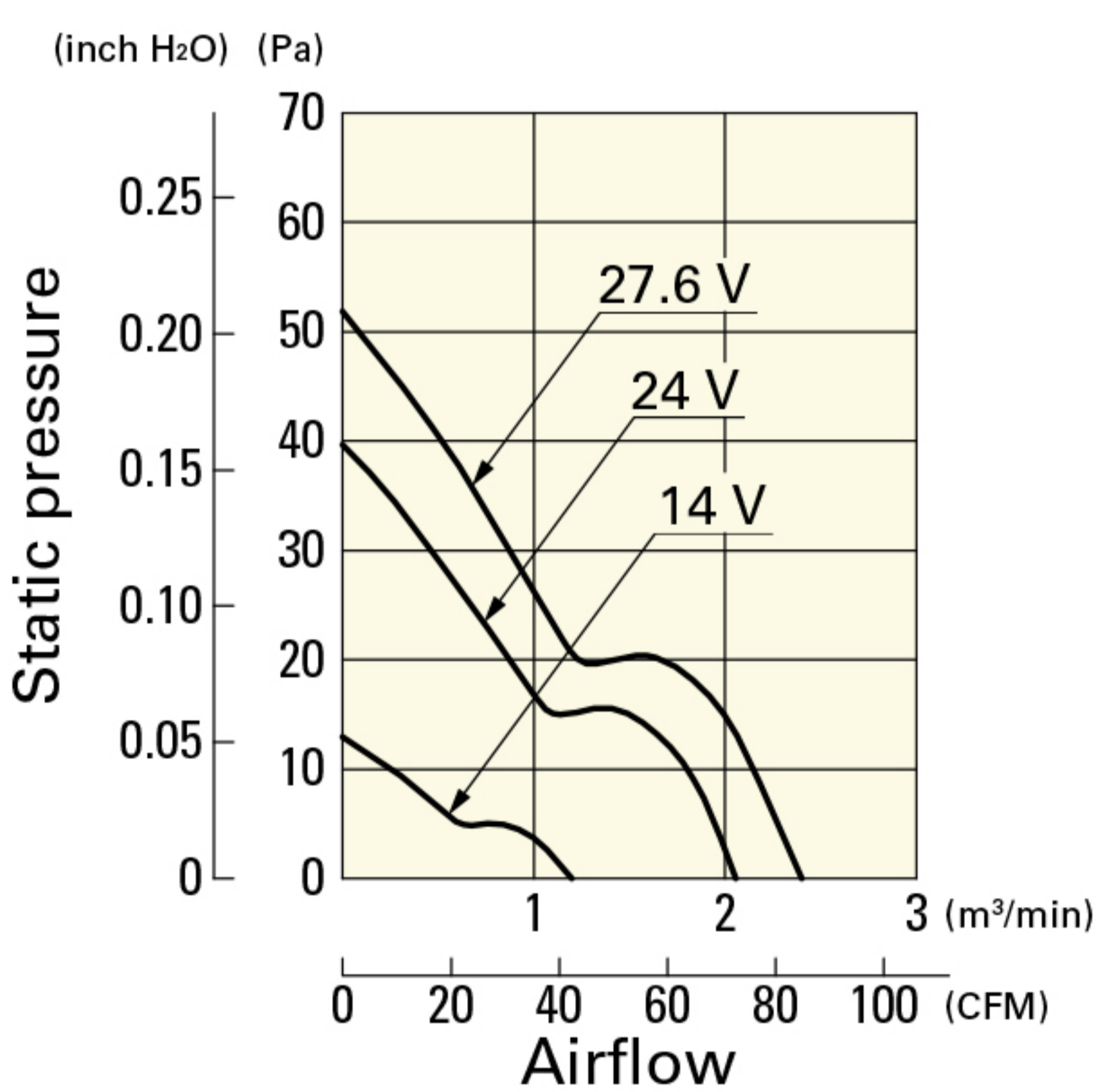
9G1248H101 With pulse sensor
