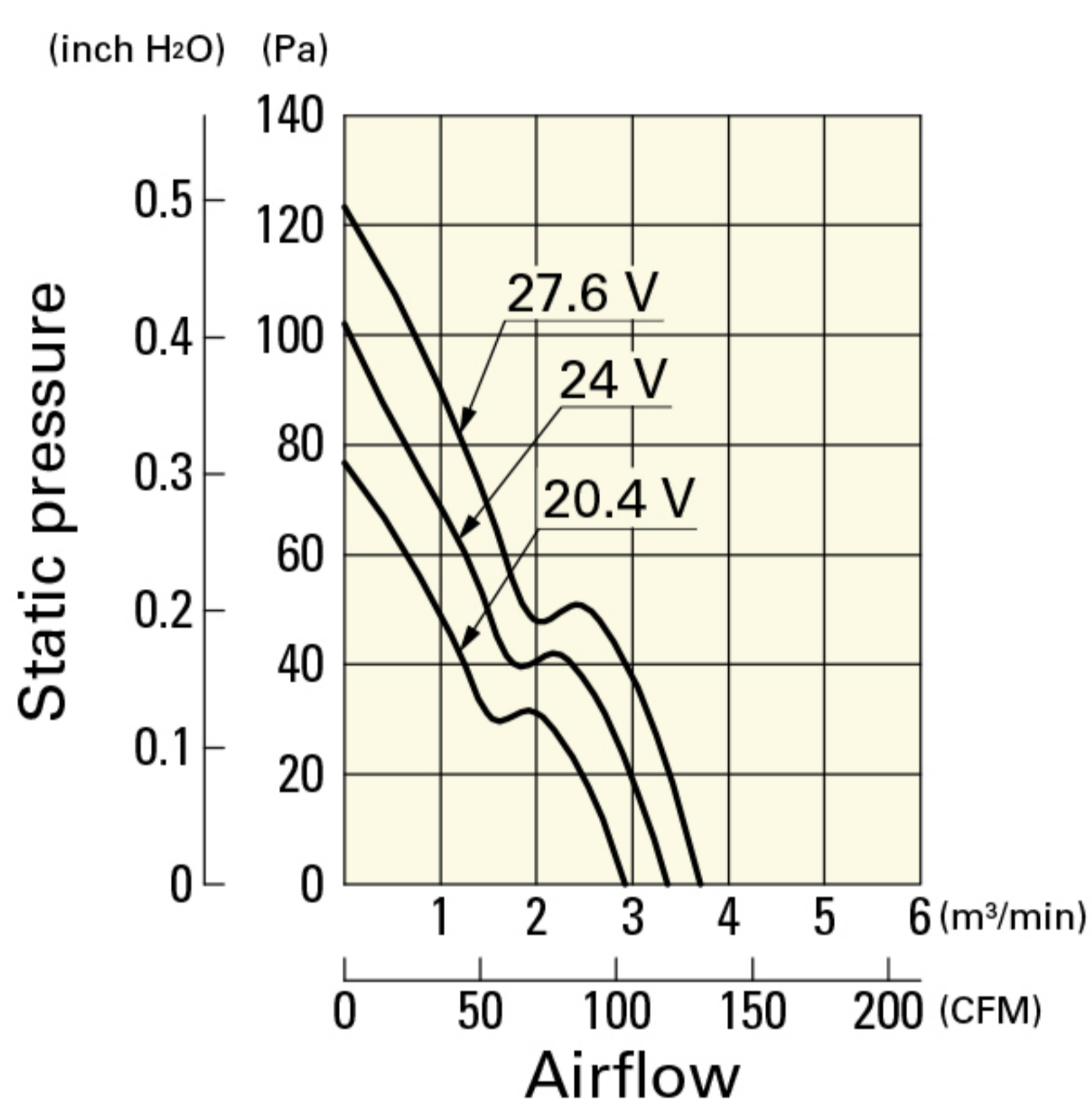
9G1224M101 With pulse sensor
