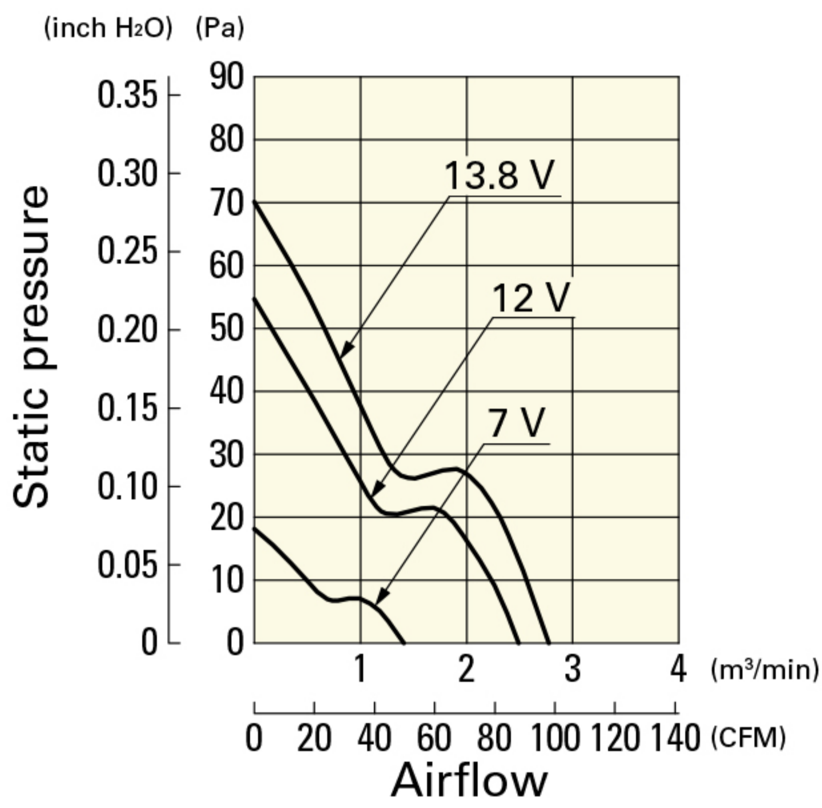
9G1224E101 With pulse sensor
