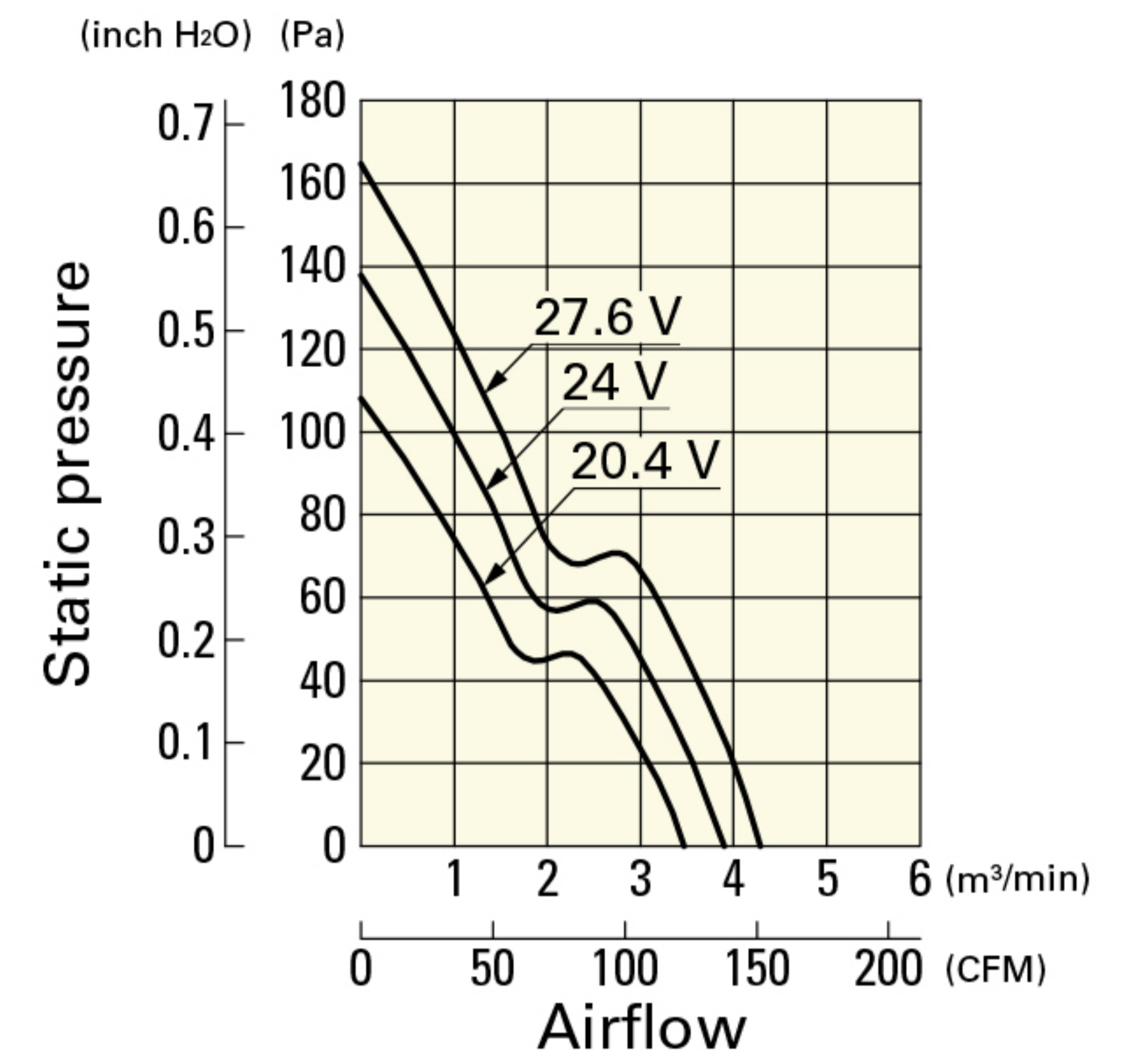
9G1224F101 With pulse sensor
