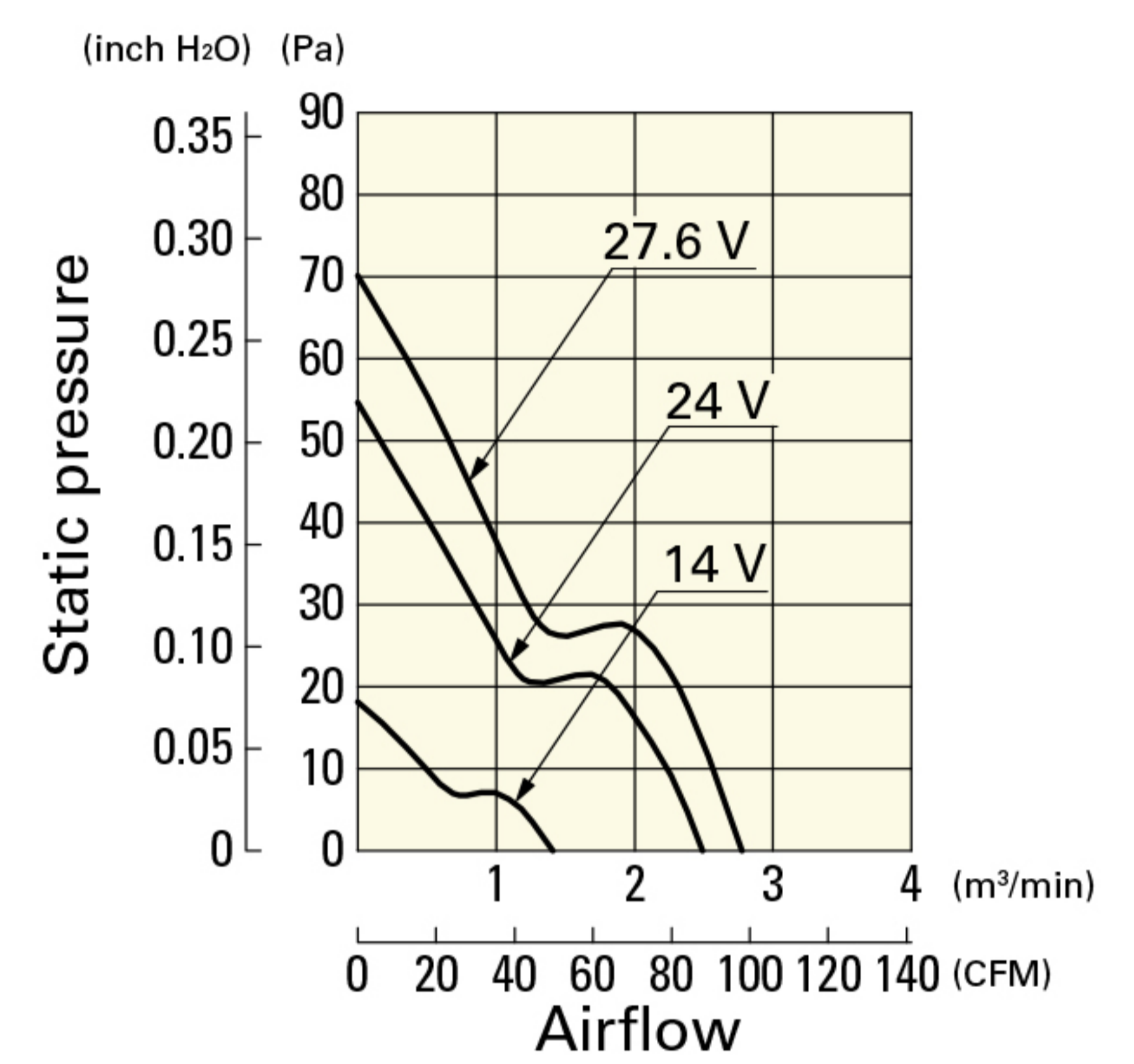
9G1248E101 With pulse sensor
