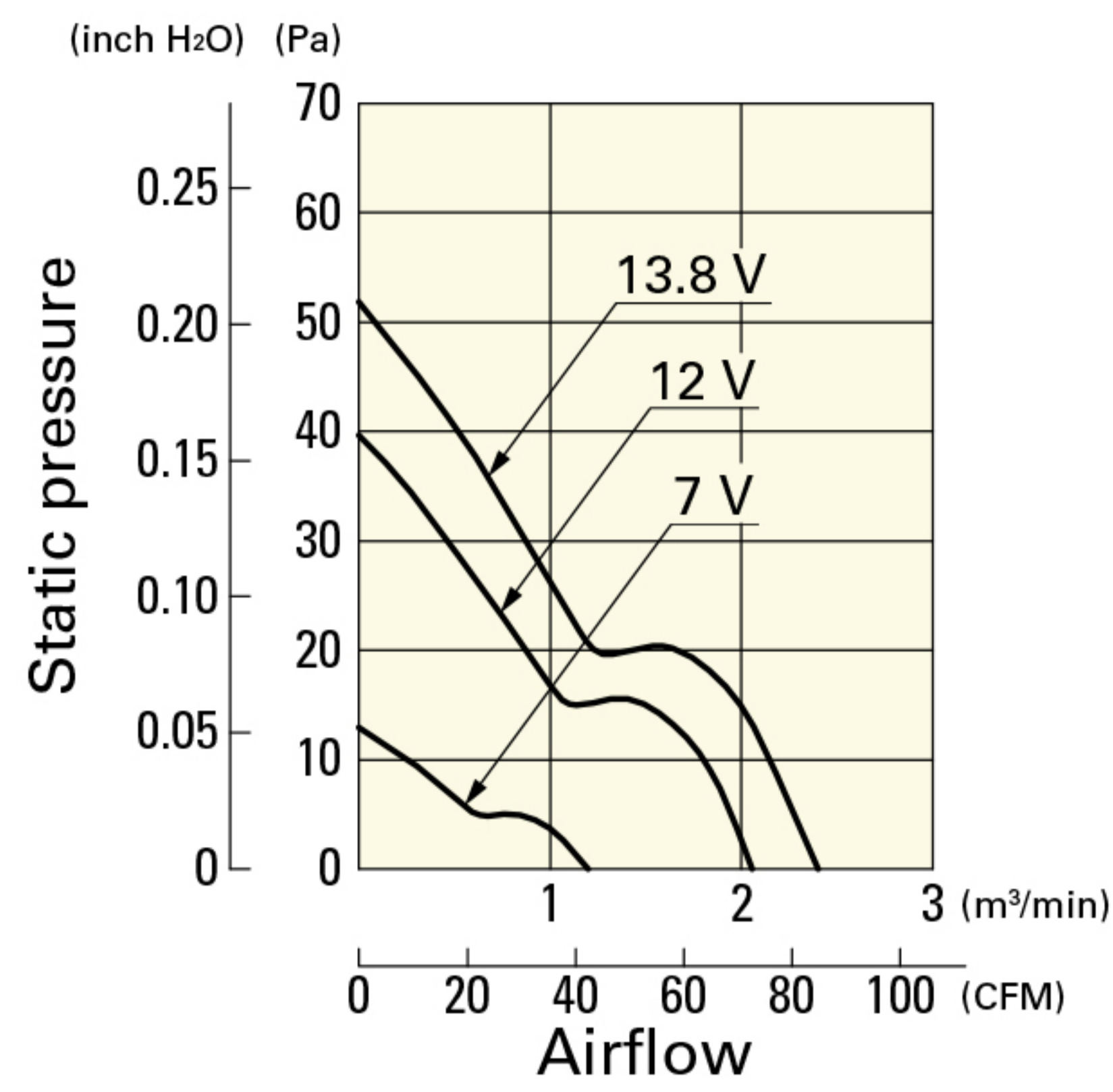
9G1224H101 With pulse sensor
