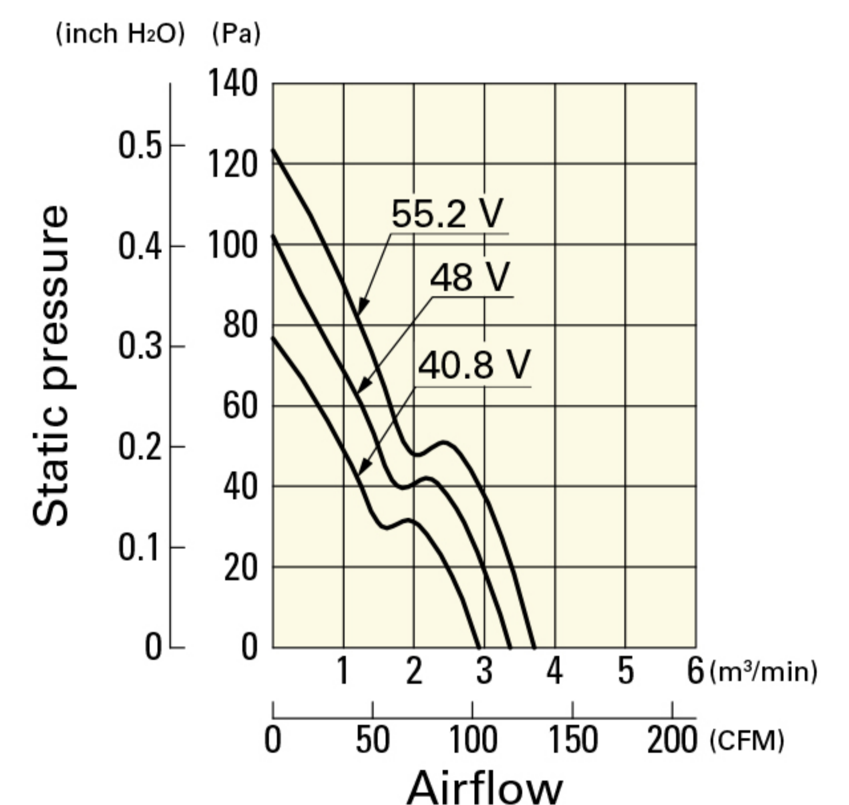
9G1248M101 With pulse sensor
