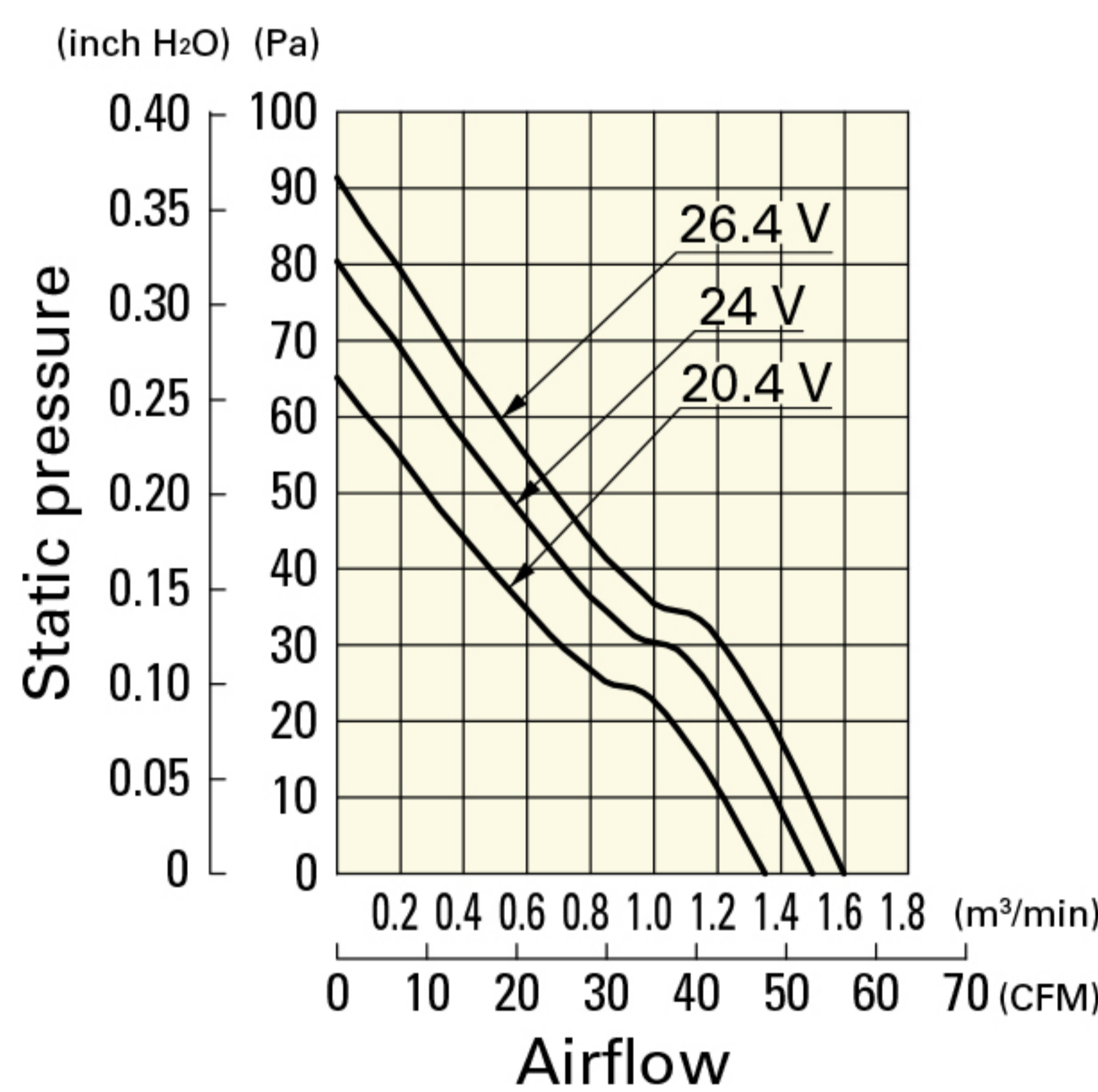
109R0824F401 With pulse sensor
