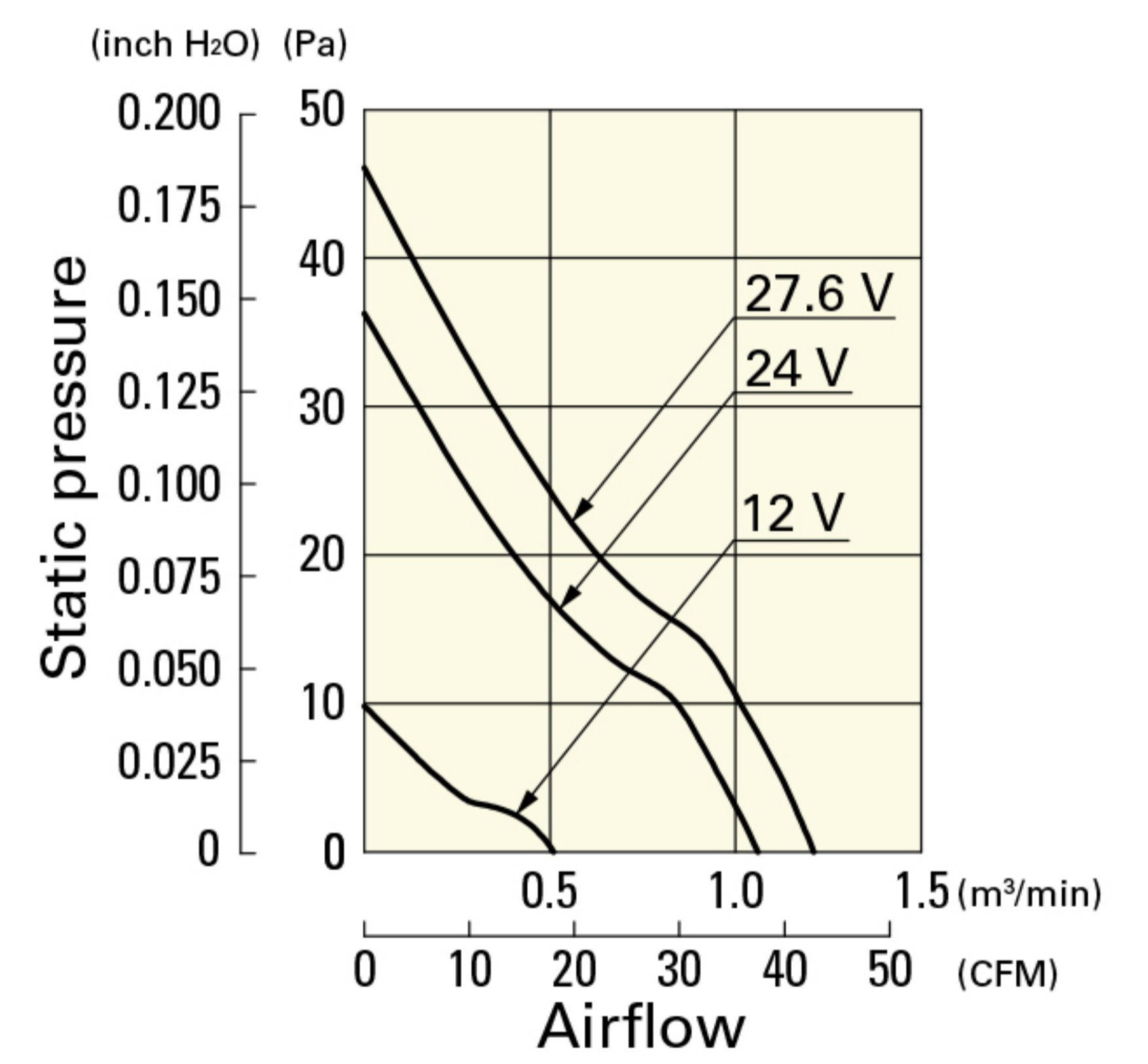
109R0824L401 With pulse sensor
