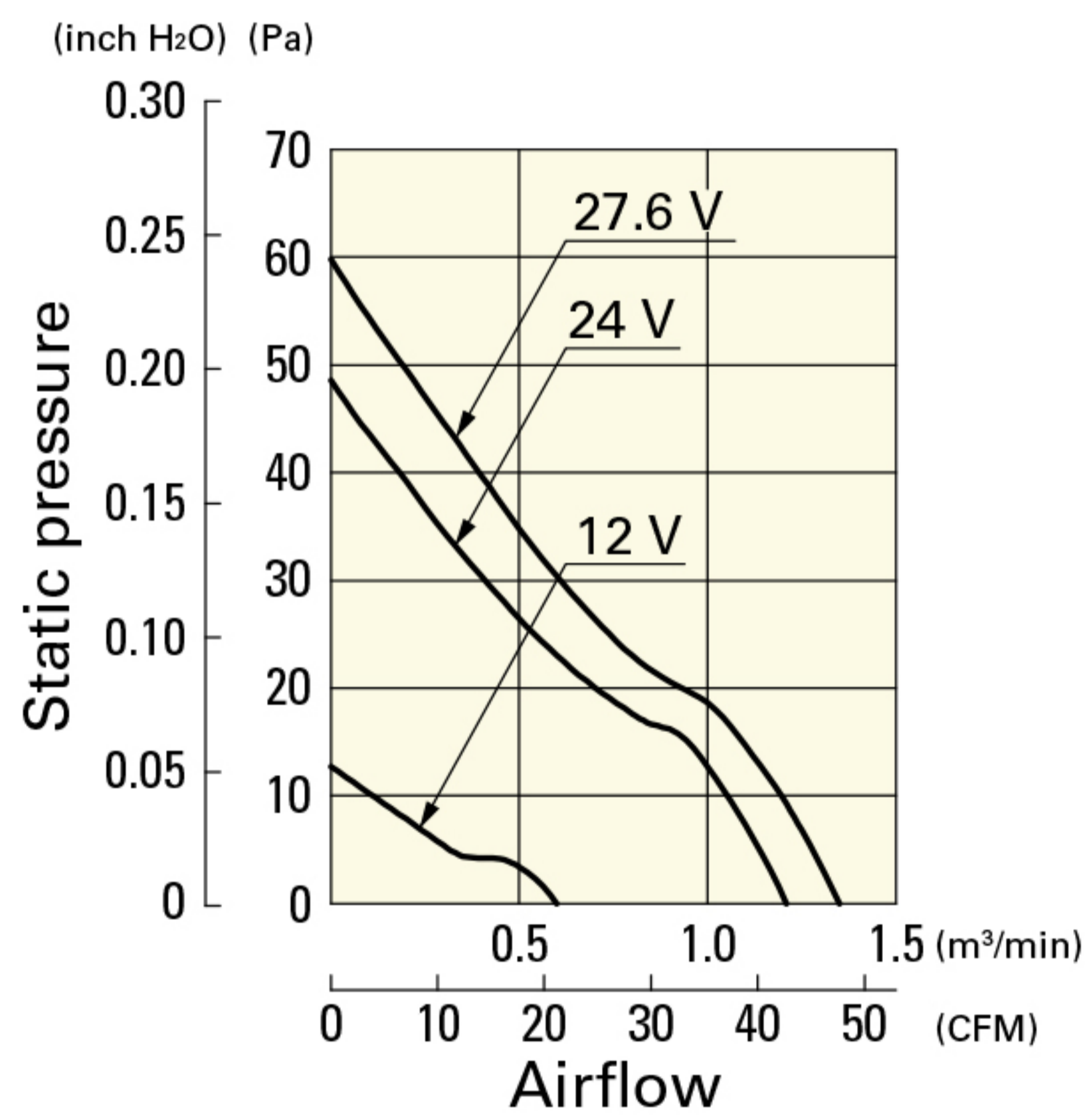
109R0824M401 With pulse sensor
