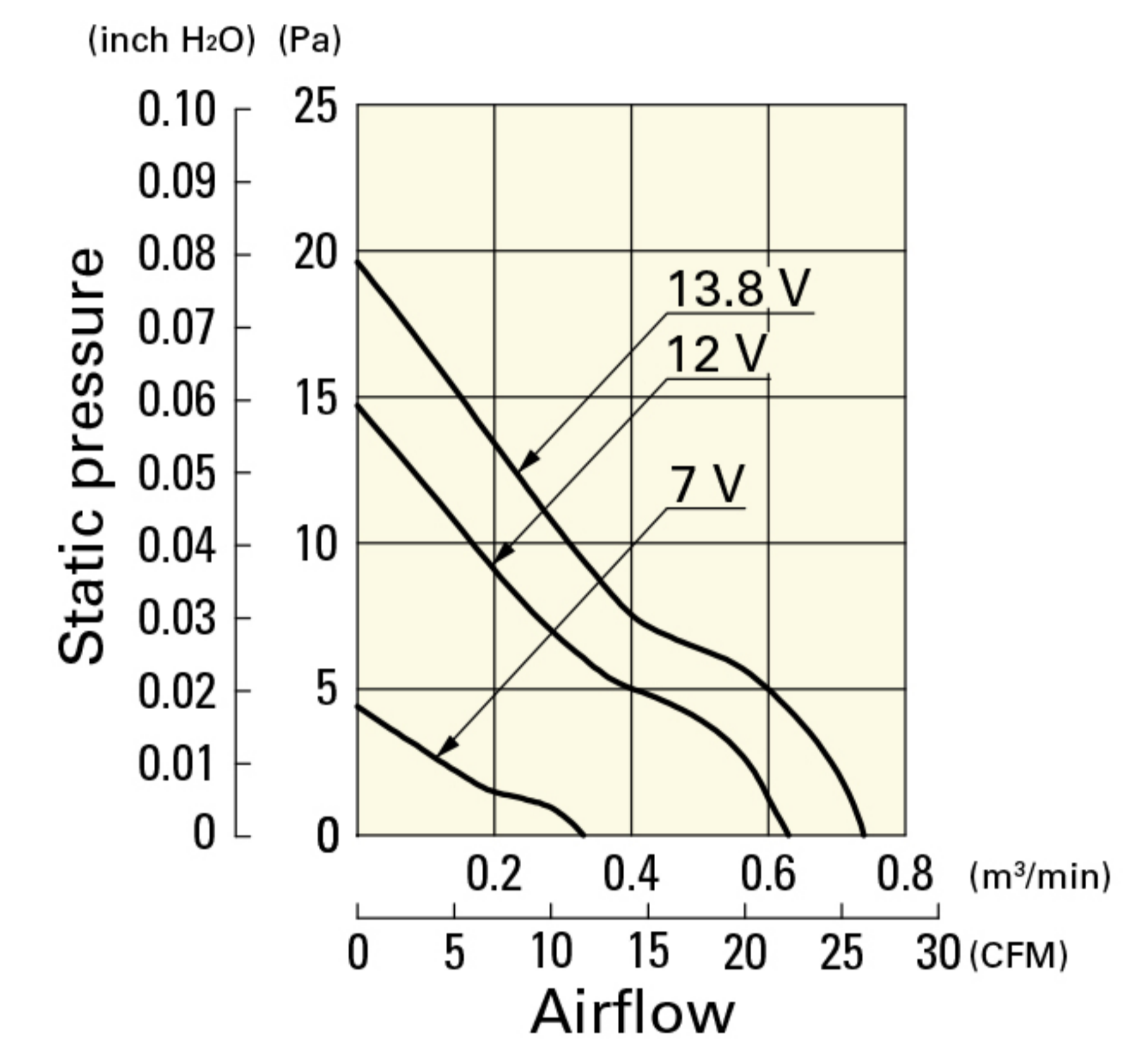
109R0824H401 With pulse sensor
