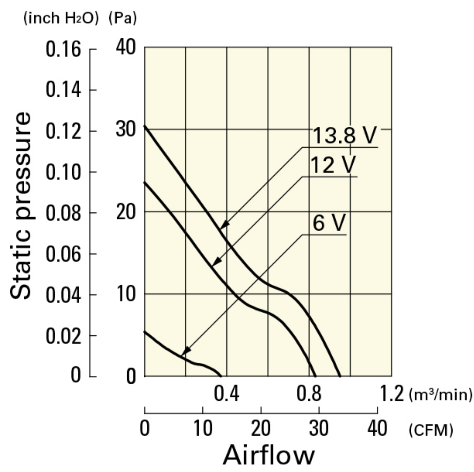
109R0824S401 With pulse sensor
