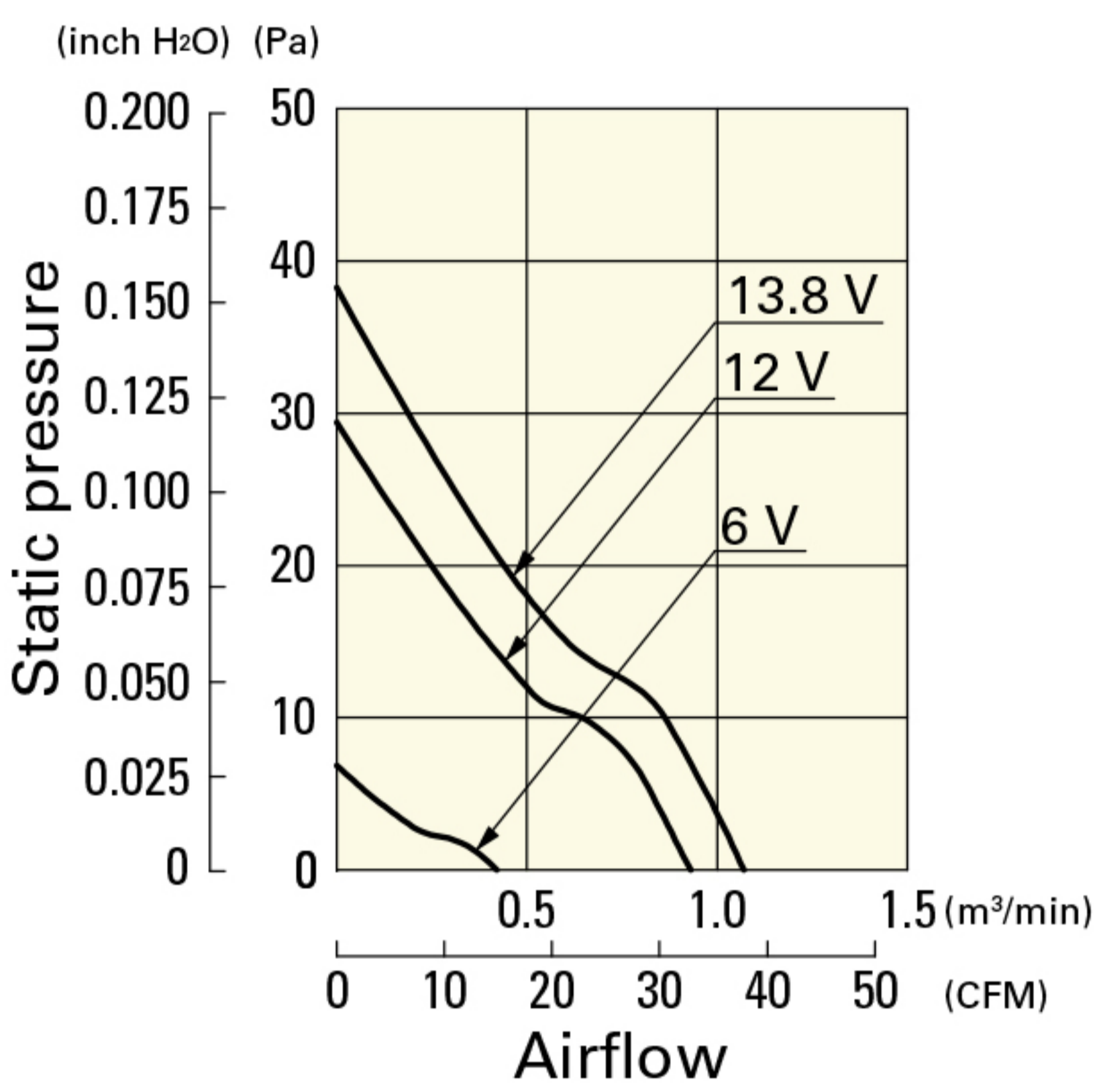
109R0824G401 With pulse sensor
