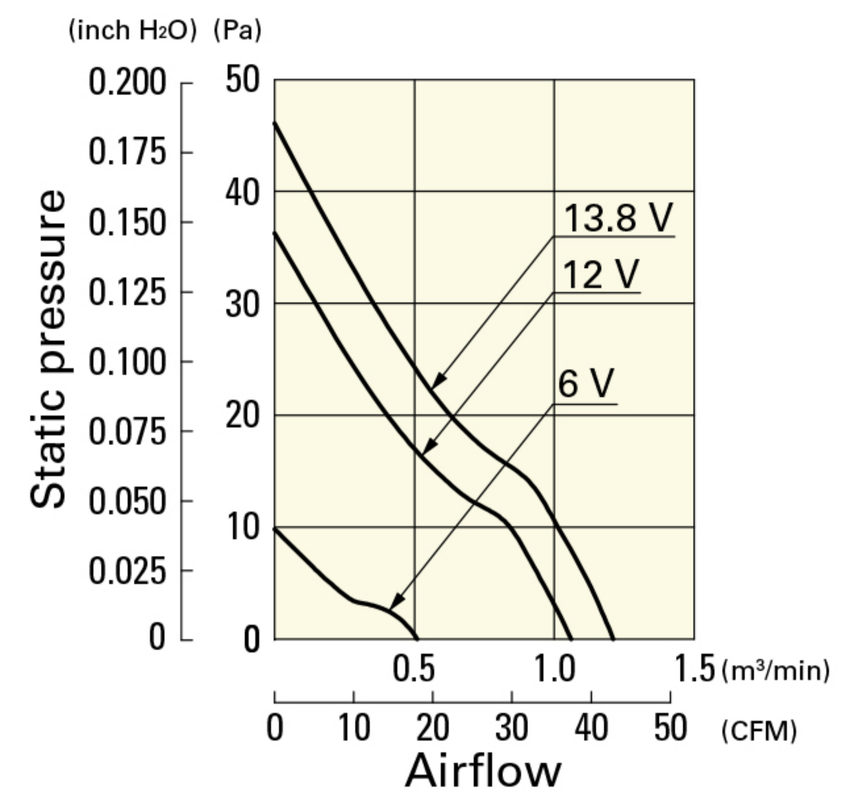
109R0812L401 With pulse sensor
