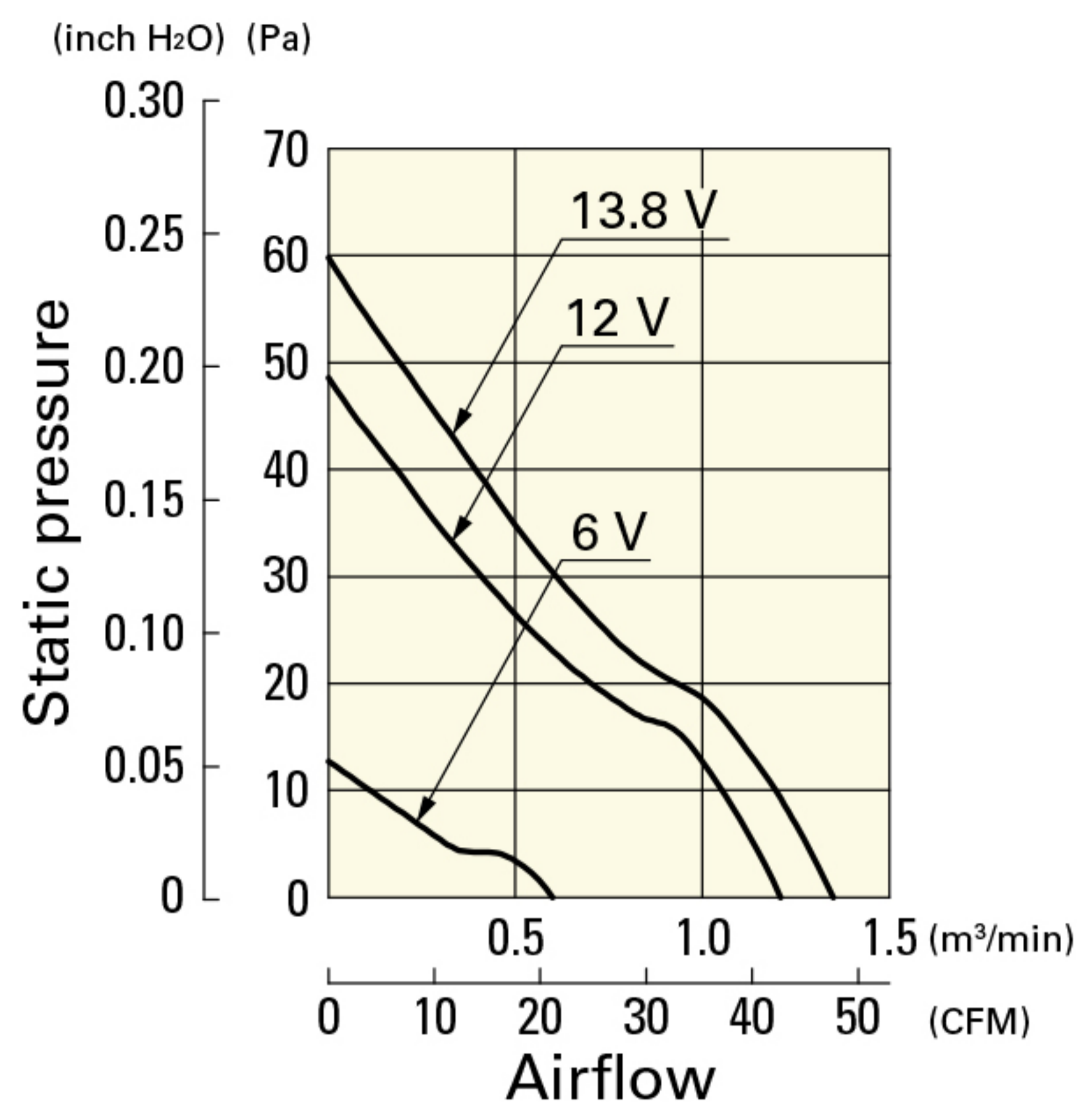
109R0812M401 With pulse sensor
