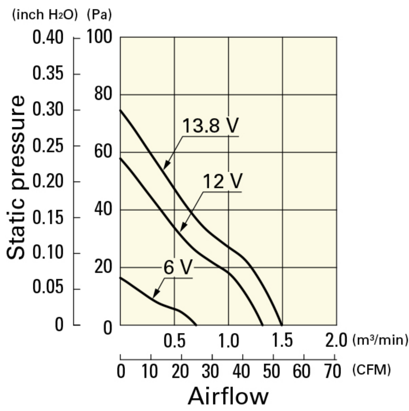
109R0812F401 With pulse sensor
