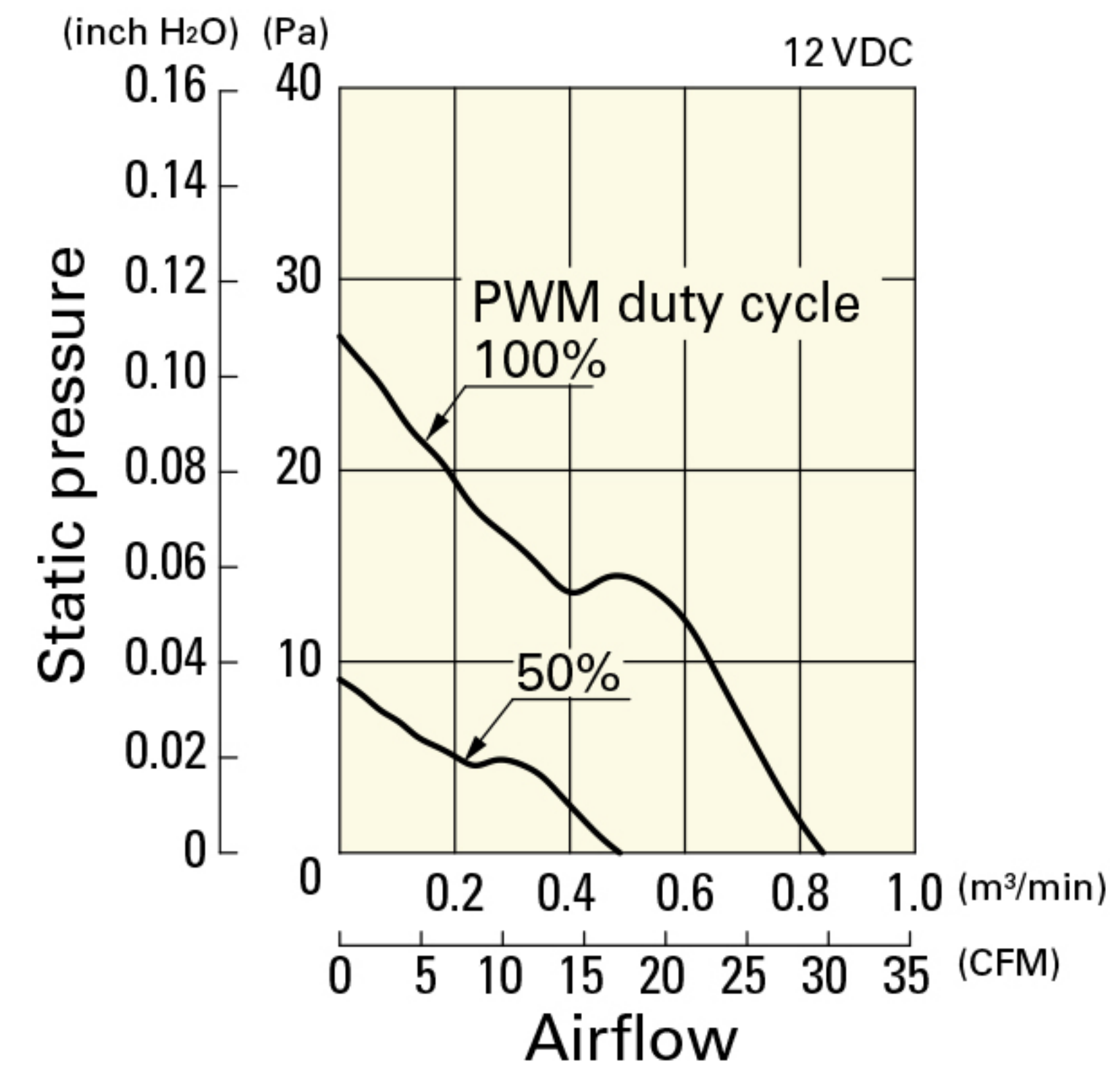
PWM duty cycle
