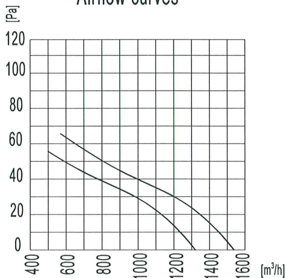
Airflow curves
