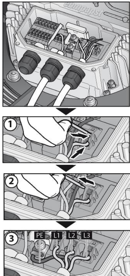
Fig. 2: Connecting wires to terminals
