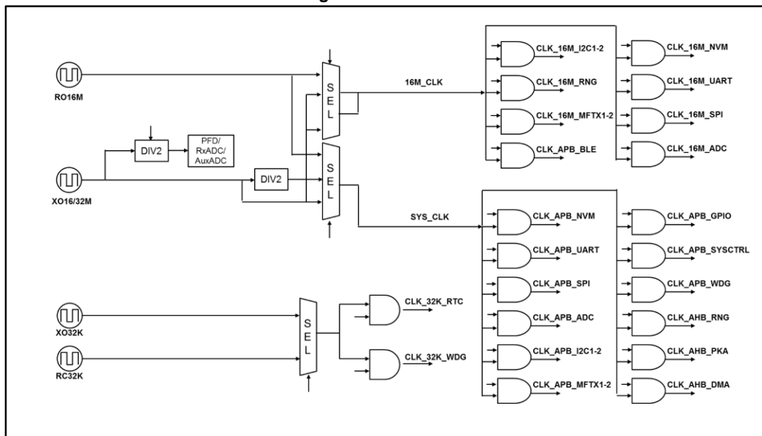
Figure 6: Clock tree
