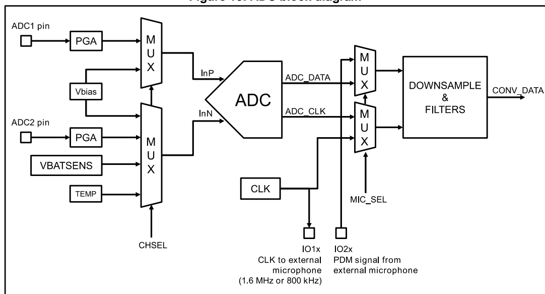
Figure 10: ADC block diagram
