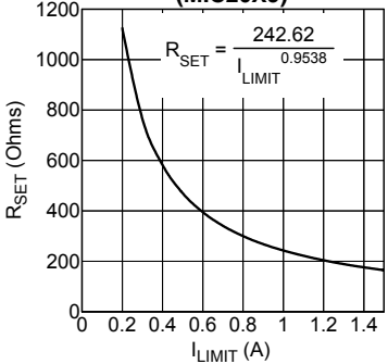
R SET vs. I LIMIT (MIC20X9)
