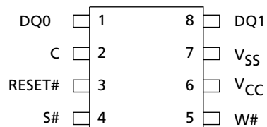
Figure 2: Pin Connections: VFQFPN and SO
