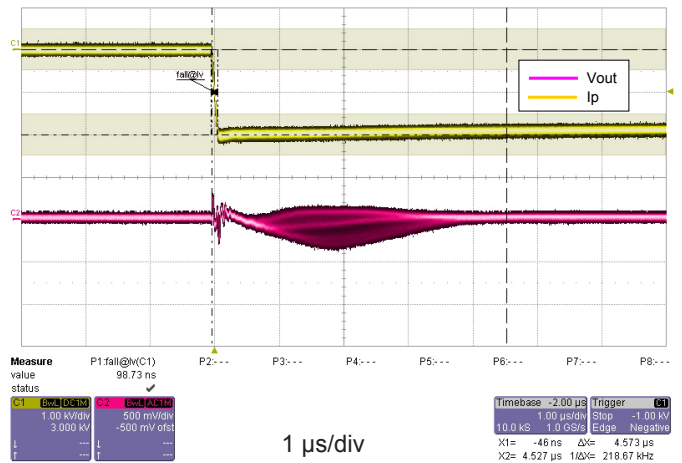
Figure 14: dv/dt
