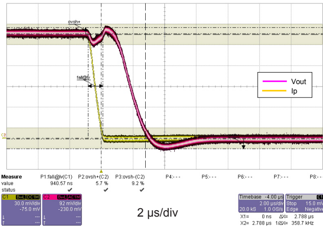
Figure 8: Step response
