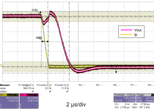
Figure 13: Step response
