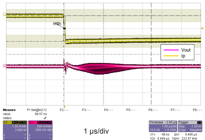
Figure 9: dv/dt
