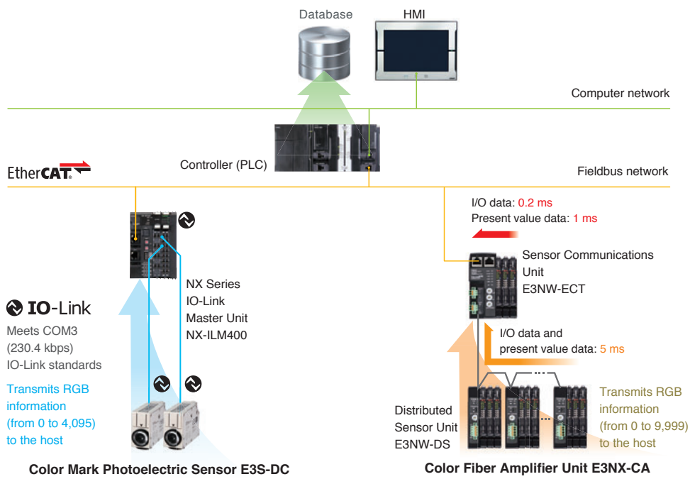
Color Mark Photoelectric Sensor (E3S-DC):
