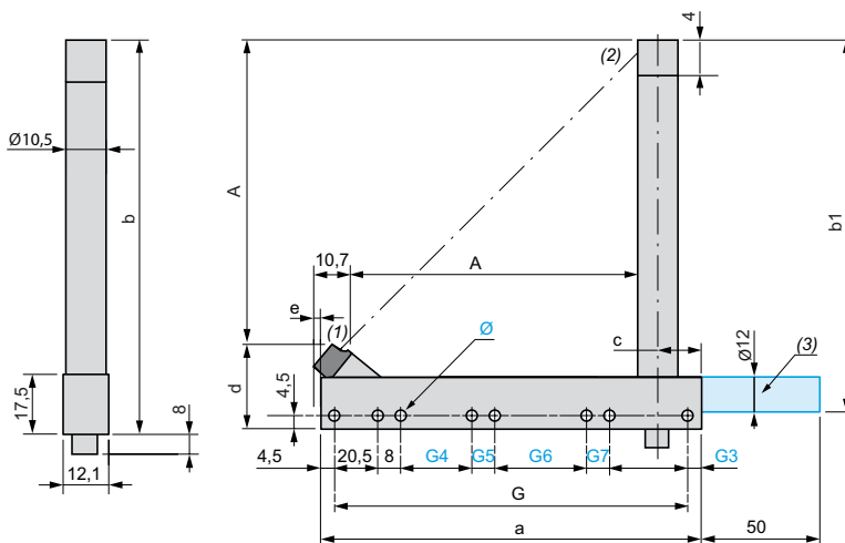
(1) Transmission LED (2) Yellow LED: output signal (3) Optional fixing rod available on request. Please consult our Customer Care Centre.
