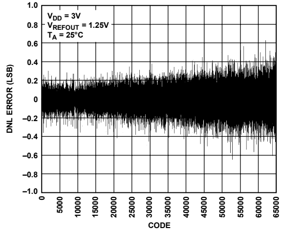
Figure 21. AD5667R DNL, 1.25 V Internal Reference
