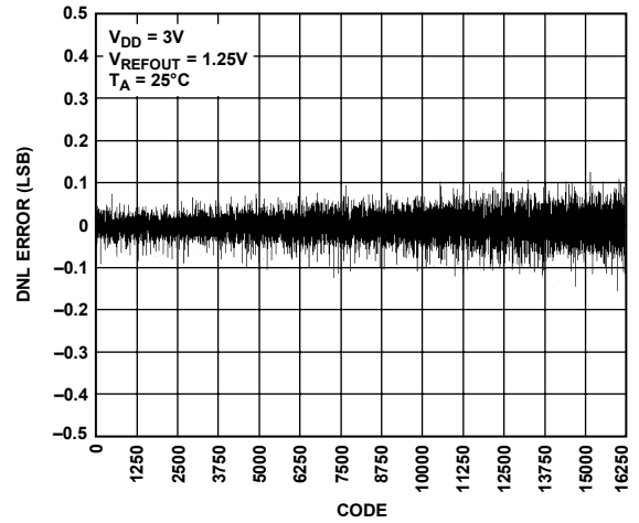
Figure 22. AD5647R DNL, 1.25 V Internal Reference
