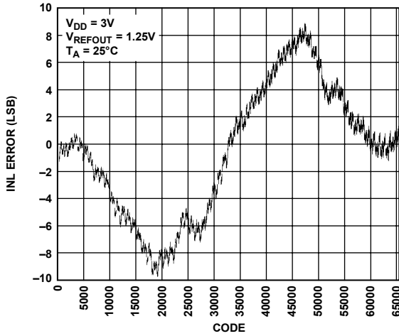
Figure 18. AD5667R INL, 1.25 V Internal Reference
