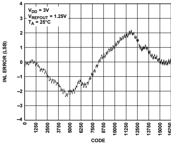
Figure 19. AD5647R INL, 1.25 V Internal Reference
