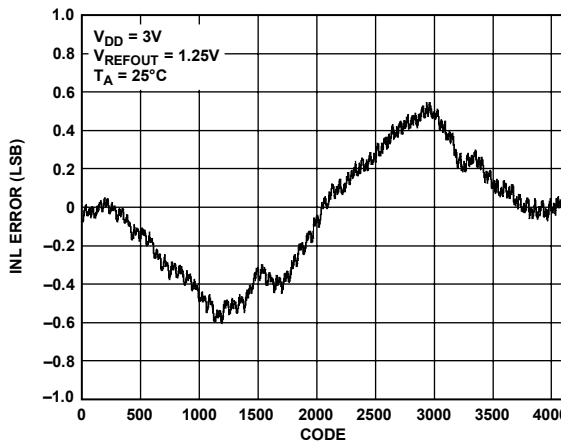
Figure 20. AD5627R INL, 1.25 V Internal Reference
