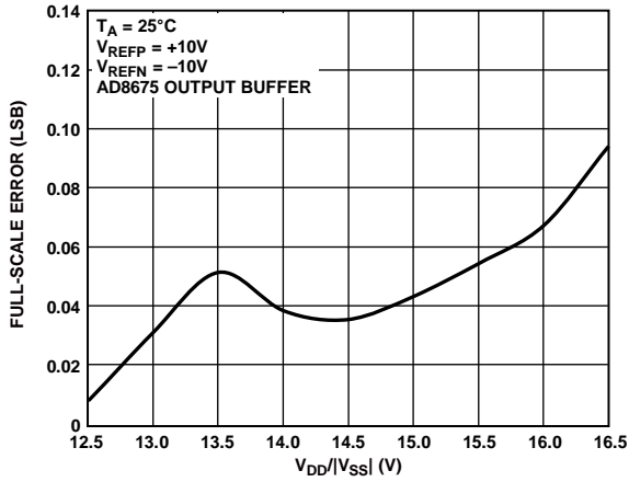
Figure 23. Full-Scale Error vs. Supply Voltage, ±10 V Span
