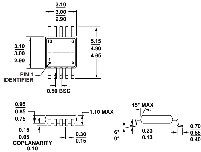
COMPLIANT TO JEDEC STANDARDS MO-187-BA Figure 53. 10-Lead Mini Small Outline Package [MSOP] (RM-10) Dimensions shown in millimeters
