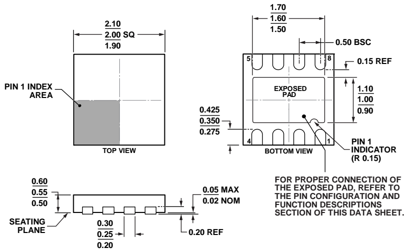
Figure 52. 8-Lead Lead Frame Chip Scale Package [LFCSP_UD] 2.00 mm × 2.00 mm Body, Ultra Thin, Dual Lead (CP-8-10) Dimensions shown in millimeters
