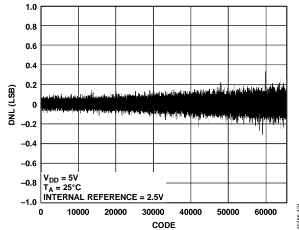
Figure 16. AD5696R DNL
