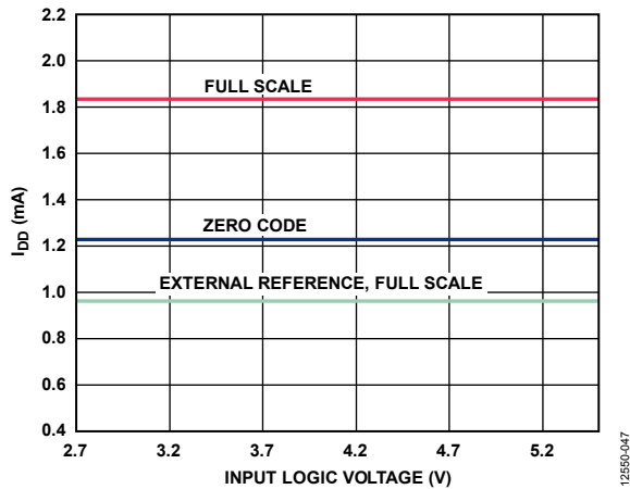
Figure 26. Supply Current ( I_{DD} ) vs. Input Logic Voltage
