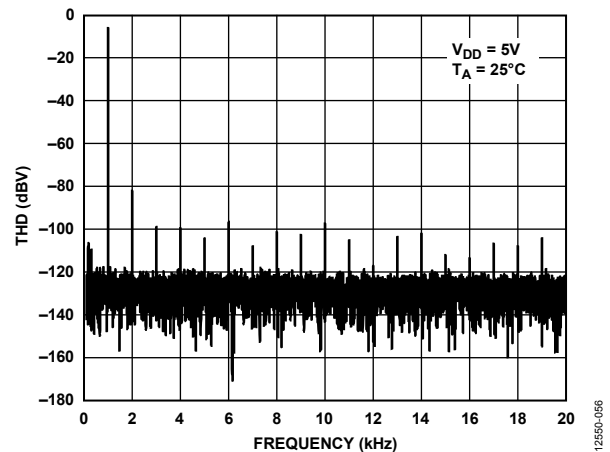
Figure 35. Total Harmonic Distortion (THD) at 1 kHz
