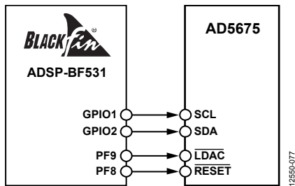
Figure 48. AD5675 to ADSP-BF531 Interface
