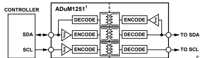
Figure 50. Isolated Interface
