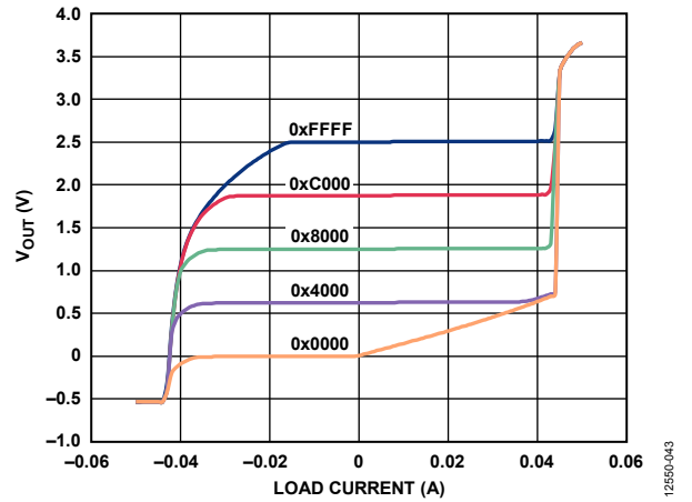
Figure 39. Multiplying Bandwidth
