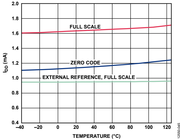
Figure 24. Supply Current ( I_{DD} ) vs. Temperature
