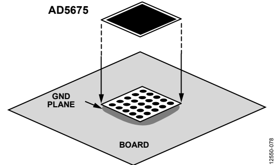
Figure 49. Pad Connection to Board
