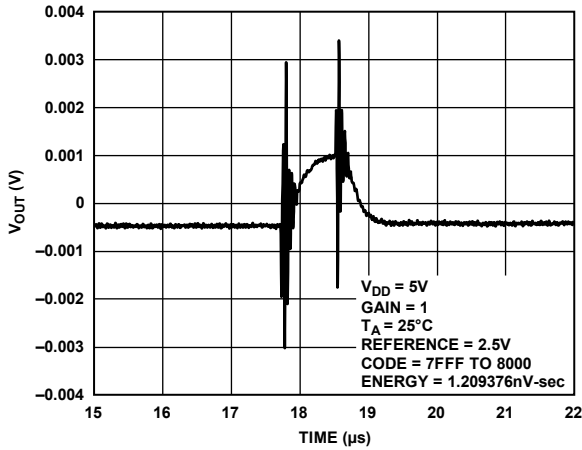
Figure 30. Digital-to-Analog Glitch Impulse
