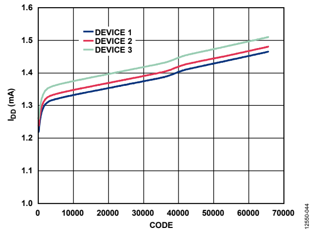
Figure 23. Supply Current ( I_{DD} ) vs. Code
