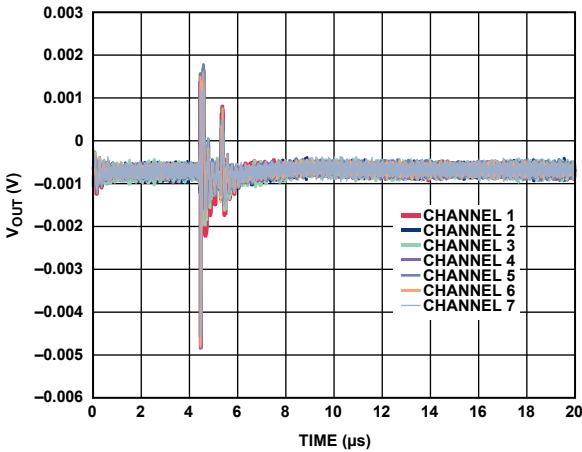
Figure 31. Analog Crosstalk
