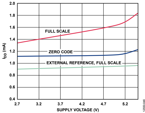
Figure 25. Supply Current ( I_{DD} ) vs. Supply Voltage
