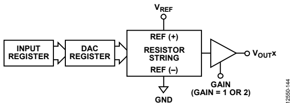
Figure 40. Single DAC Channel Architecture Block Diagram
