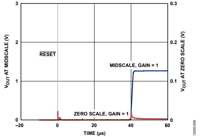
Figure 38. Hardware Reset
