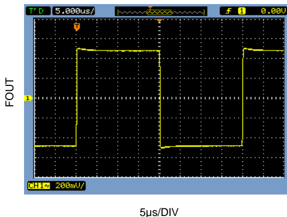
FOUT Transient Response V_{DD} = 1V , BOOST = V_{DD} , C_{LOAD} = 47pF
