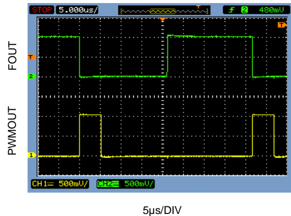
FOUT and PWMOUT Transient Response V_{DD} = 1V , V_{CNTRL} = 0.035 \times V_{DD} , BOOST = V_{DD} , C_{LOAD} = 22pF
