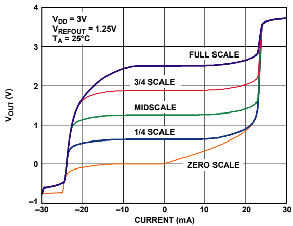
Figure 35. AD56x4R-3 Source and Sink Capability
