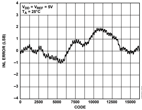
Figure 5. AD5644R INL, External Reference
