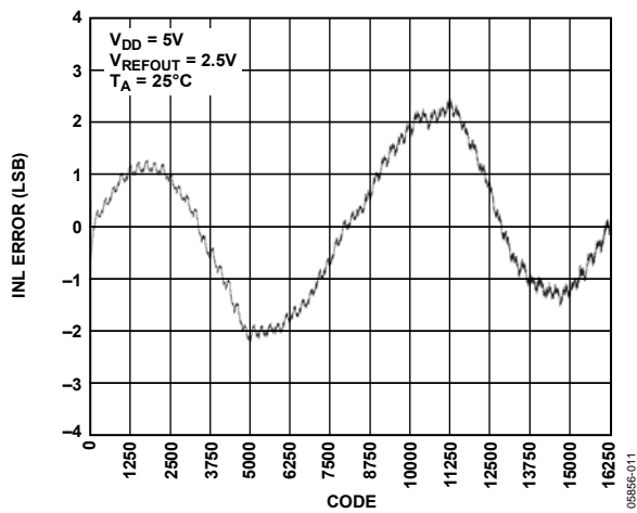
Figure 11. AD5644R-5 INL, Internal Reference
