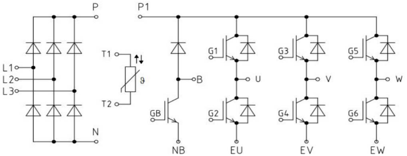
Figure11. Circuit Diagram
