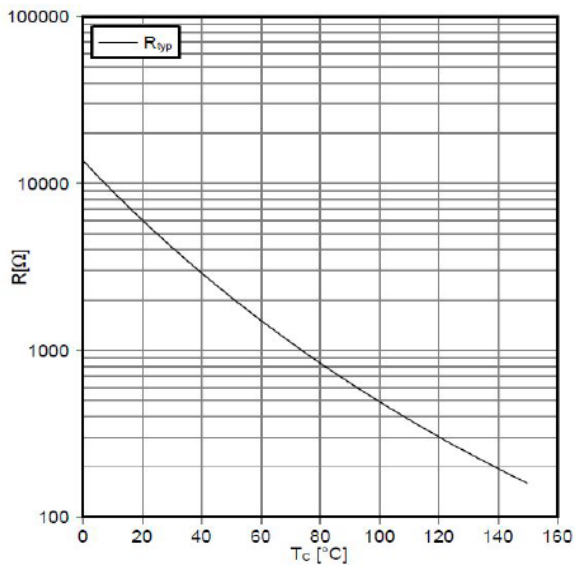
Figure11. NTC-Thermistor-temperature characteristic
