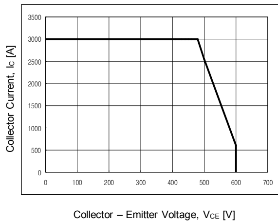
Fig 10. SCSOA characteristics
