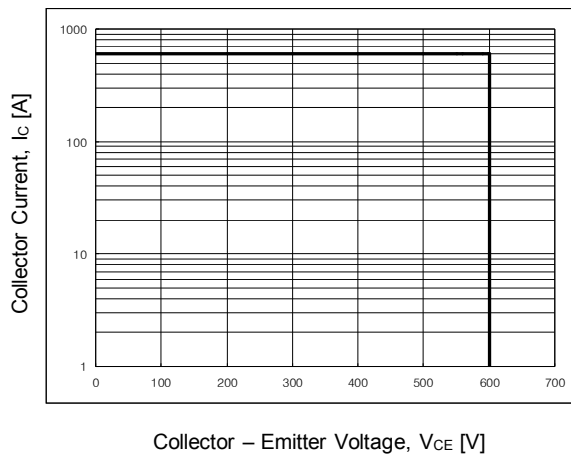
Fig 9. RBSOA characteristics
