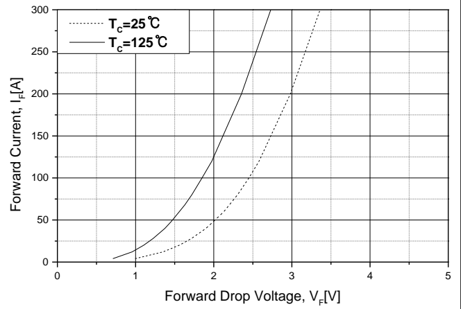
Fig.10 Forward Characteristics
