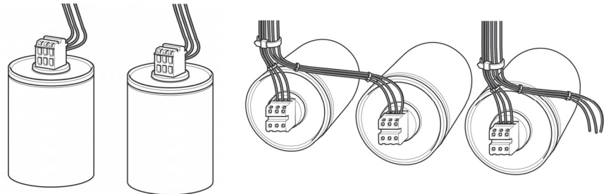
Figure 2: PhaseCap and PhaseCap Compact in vertical or horizontal mounting position.
