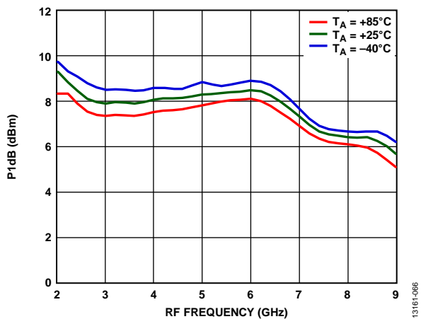
Figure 70. Input P1dB vs. RF Frequency at Various Temperatures, LO Drive = 15 dBm
