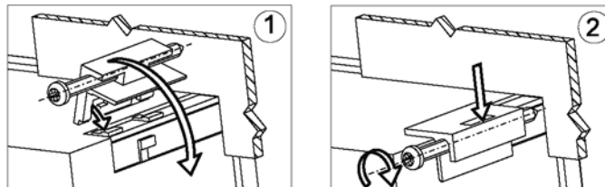
Fig. 1. Meter fitting.
