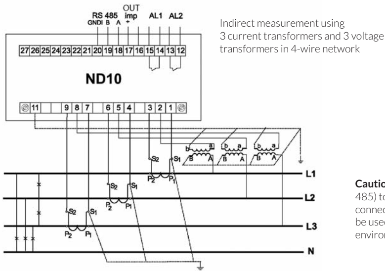
Fig 3. Connection diagrams of the meter in the 4-wire network.
