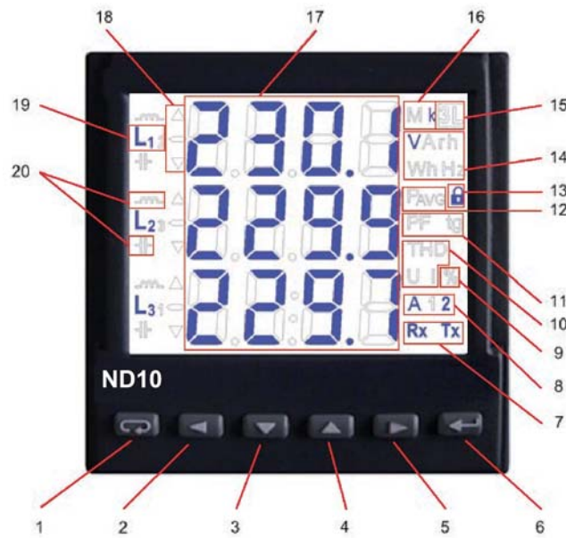
Fig. 4. Front panel.
