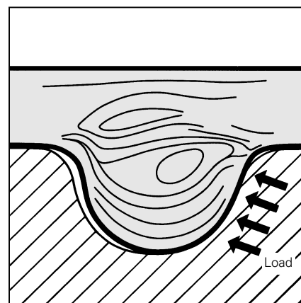
Stress distribution in the CONTI SYNCHROBELT® HTD tooth
