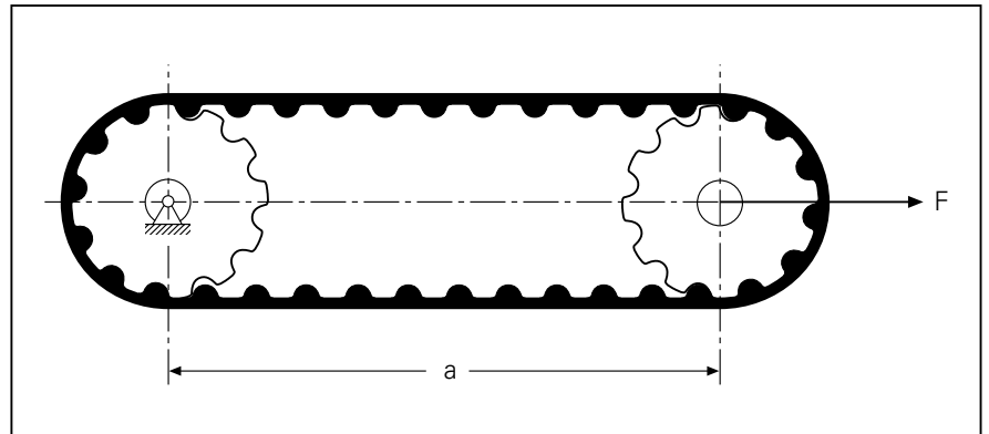
Measuring configuration
