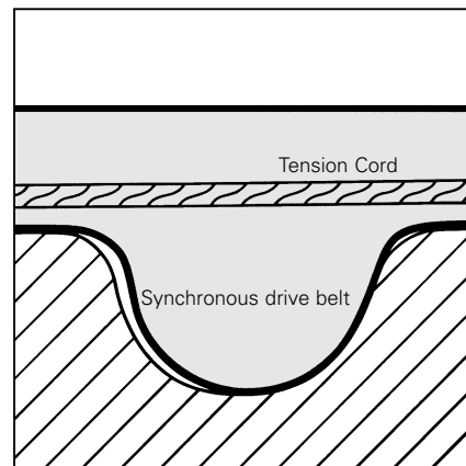
CONTI SYNCHROBELT® HTD tooth profile
