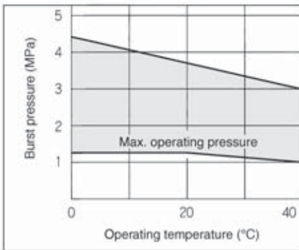
Burst Pressure Characteristics Curve
