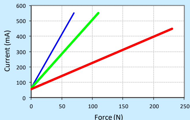
Current Curves
