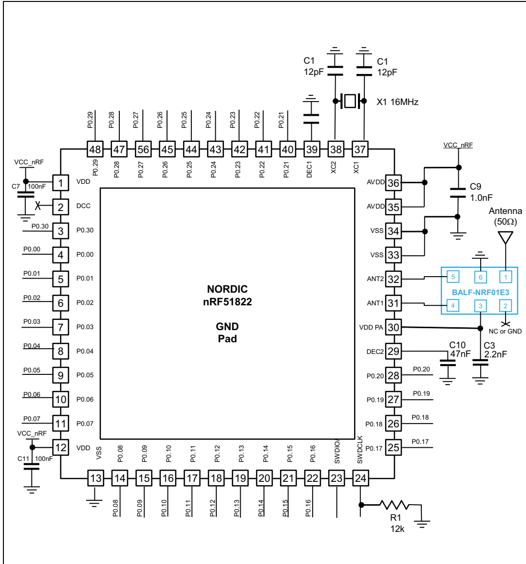
Figure 8. Application schematic
