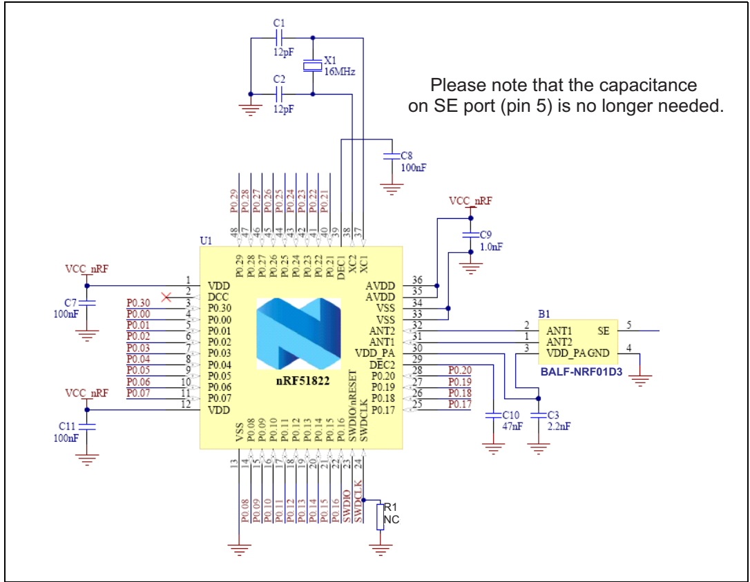
Figure 9. Application schematic
